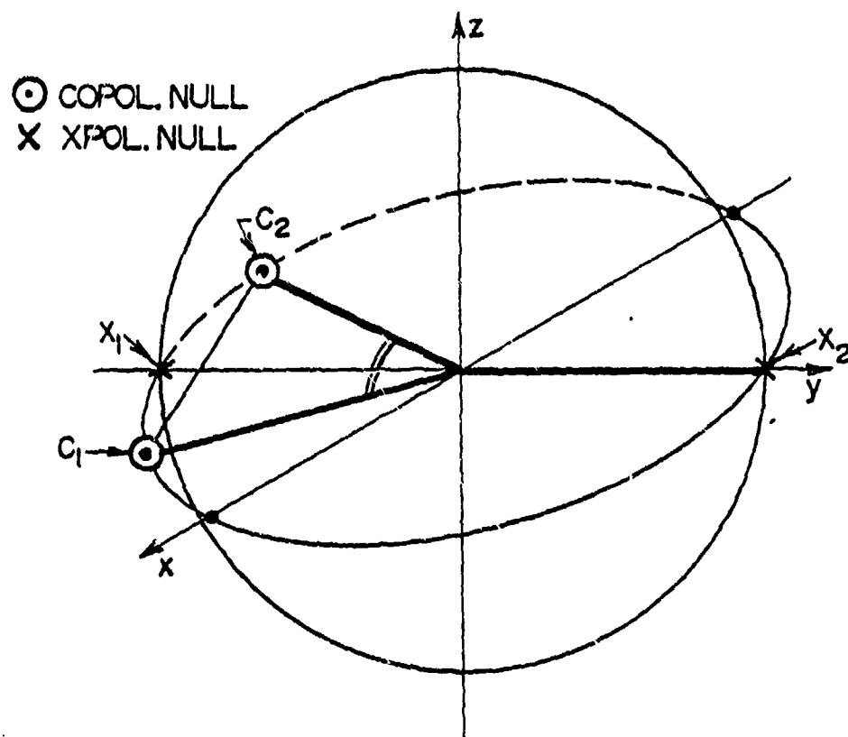
Fig. 3.14 : The Polarization Fork (Huynen 1970).
