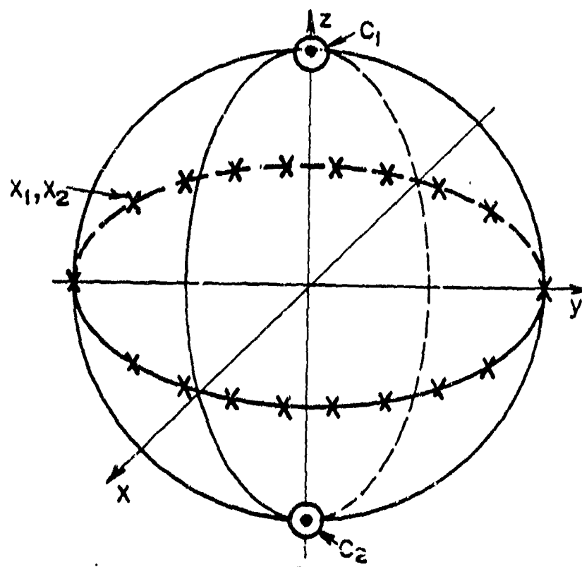
Fig. 4.2 : COPOL and XPOL nulls for a metallic sphere or flat plate.
