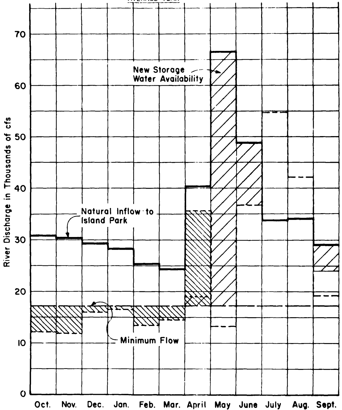
Figure A-2-3. Graphical Study Showing When New Storage Operations Would Occur- Main Stem Henrys Fork Snake River - 1951 Average Year Conditions.
