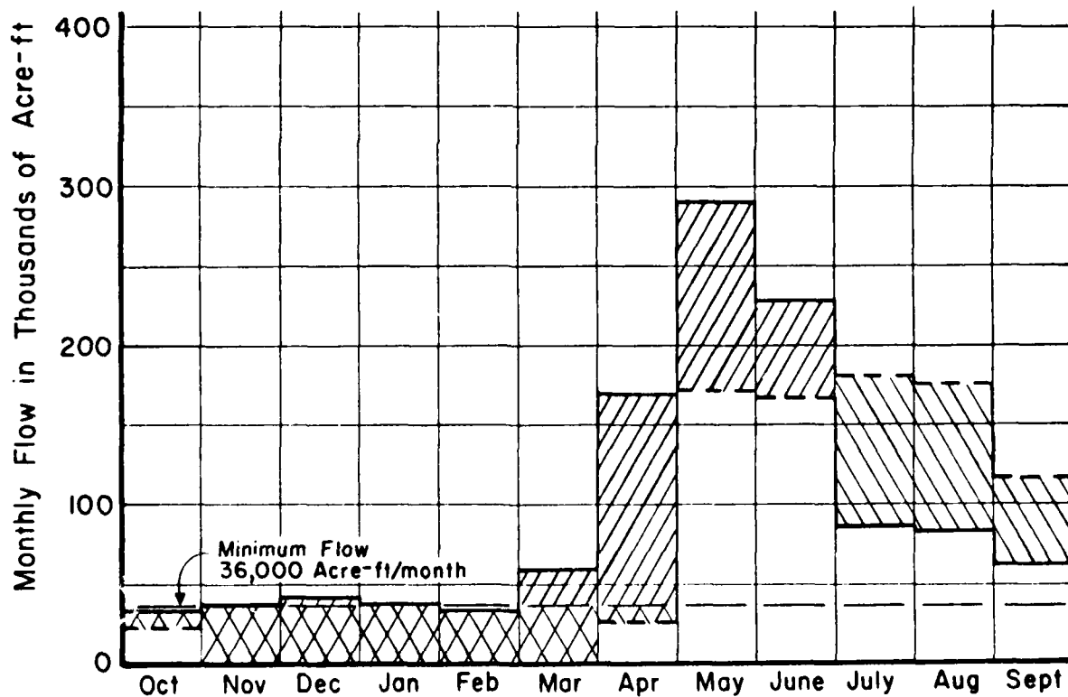
Figure A-3-2. Graphical Presentation of the Availability of Payette River Water at Horseshoe Bend (Dry Year 1977 With Actual Diversions).
