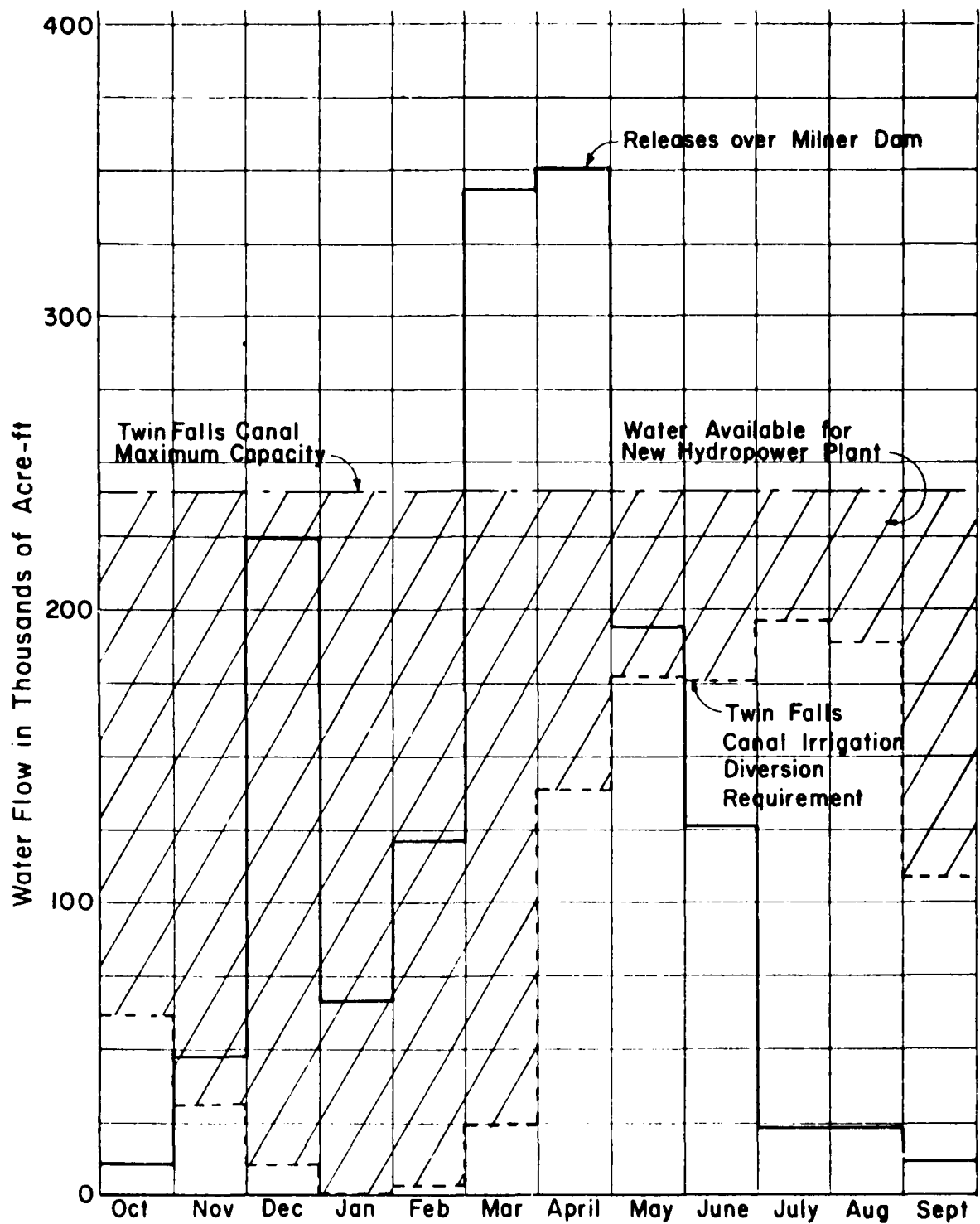
Figure 8. Monthly Hydrograph of Possible Water Release at Milner Dam on the Snake River for Possible Power Development.
