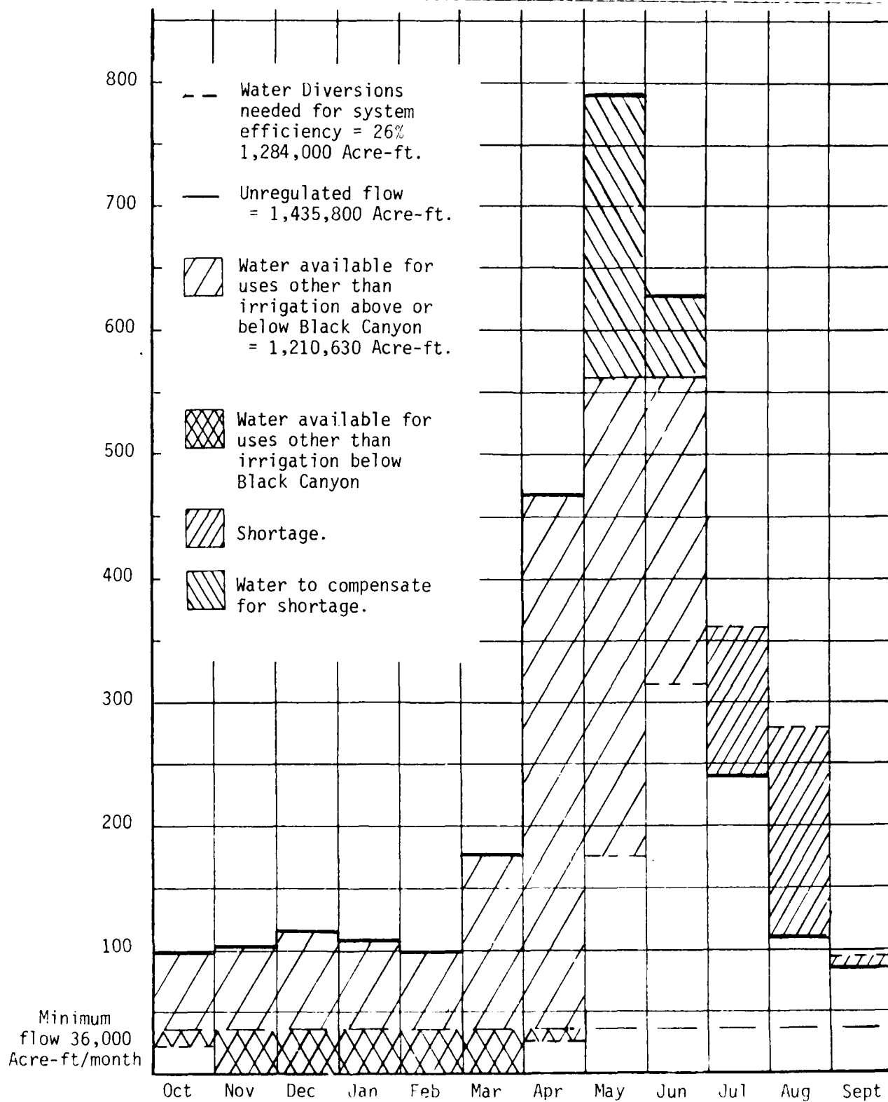
Figure A-3-6. Graphical Presentation of the Availability of Payette River Water at Horseshoe Bend (Wet Year 1951 with 26% Irrigation Efficiency).
