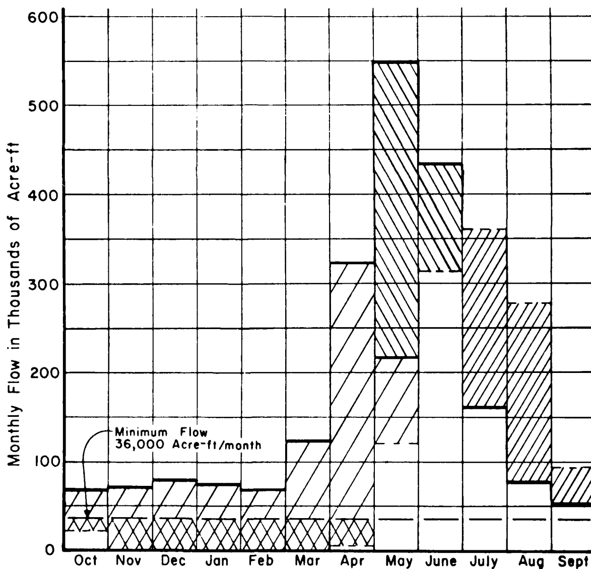
Figure A-3-5. Graphical Presentation of the Availability of Payette River Water at Horseshoe Bend (1959 Average Year with 26% irrigation efficiency).
