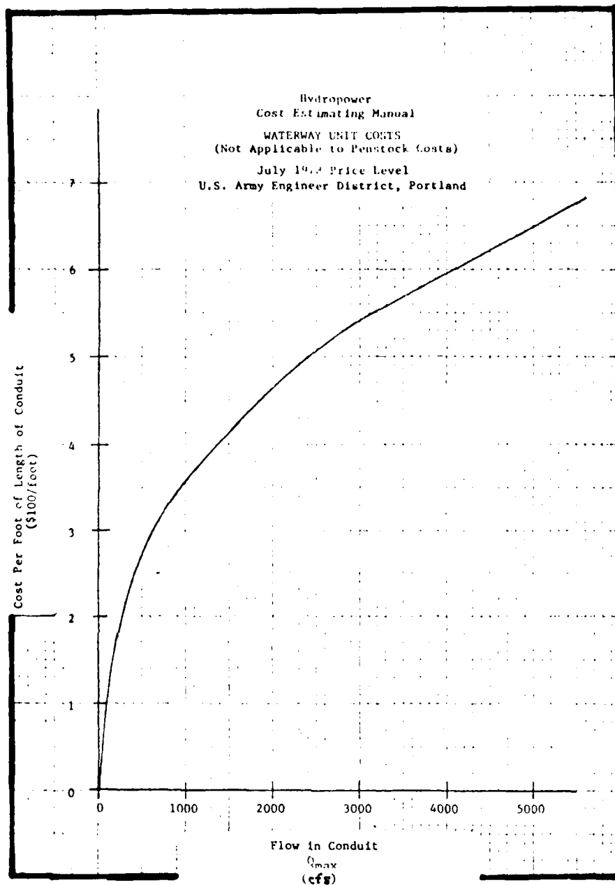
Figure A-5-4. Waterway Cost Estimating Curve.
