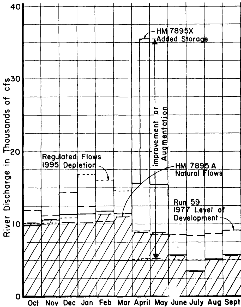
Figure 7. Monthly Hydrographs Showing Operational Characteristics of Snake River Releases From Brownlee Reservoir for Corps of Engineers Hypothetical Plan to Augment River Flows for Fishery Enhancement (1931 Dry Year).
