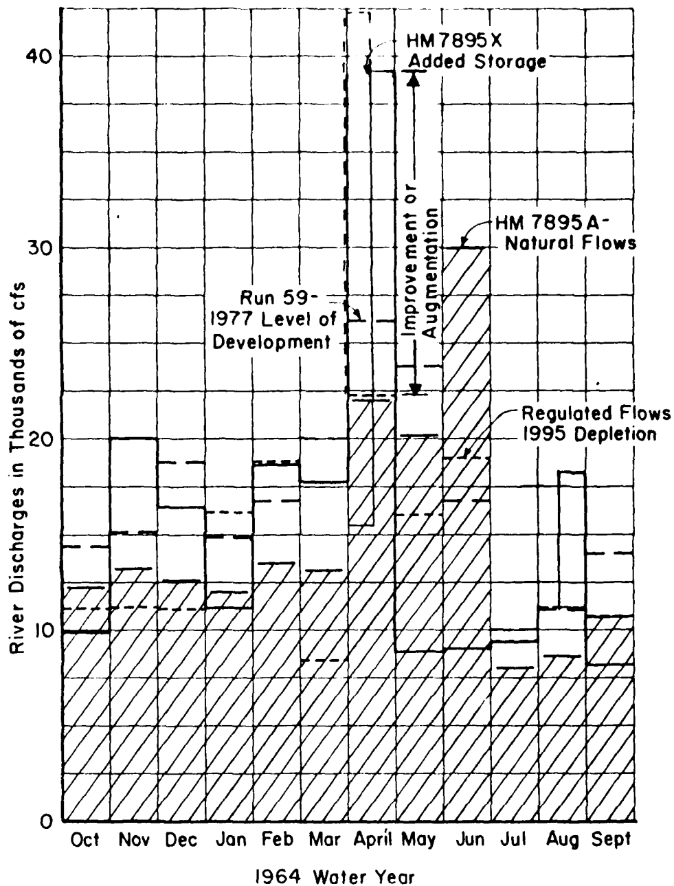
Figure 6. Hydrographs of River Discharges from Brownlee Reservoir, Snake River, Idaho Showing Operational Releases for Corps of Engineers. Hypothetical Plan to Augment River Flow for Enhancement of Fishery (1964 Average Year).
