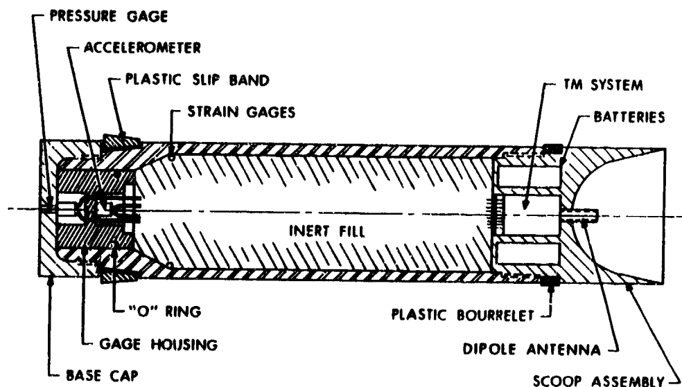
CLGP WARHEAD BODY TYPE T
