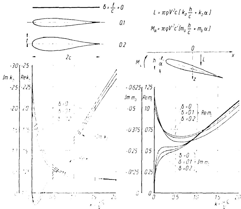
Figure 5: Influence of thickness on lift and moment coefficients of a Joukowski-profile pitching about its mean chord ( Ma = 0 ).
