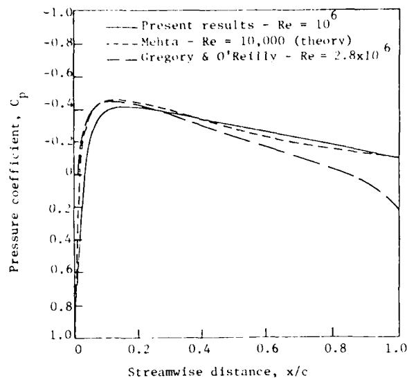
Figure 2. - Surface pressure distribution for NACA 0012 airfoil at zero incidence (full airfoil calculation)
