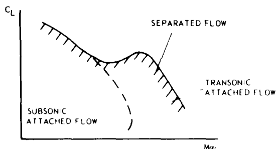
Fig. 1 Types of flow in the M_\infty - M_\infty^2 plane of similarity
