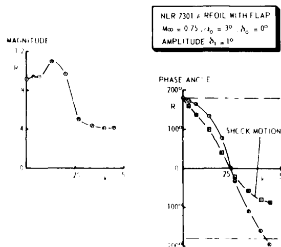
Fig. 15 Effect of boundary layer effect vector on unsteady lift and moment coefficients
