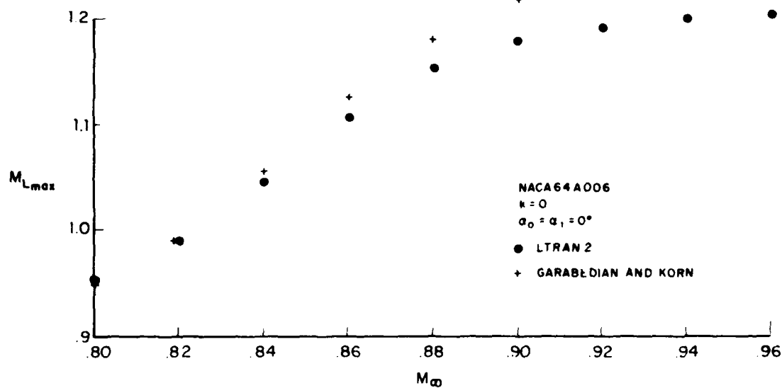
Fig.III-11(b) Maximum local Mach number
