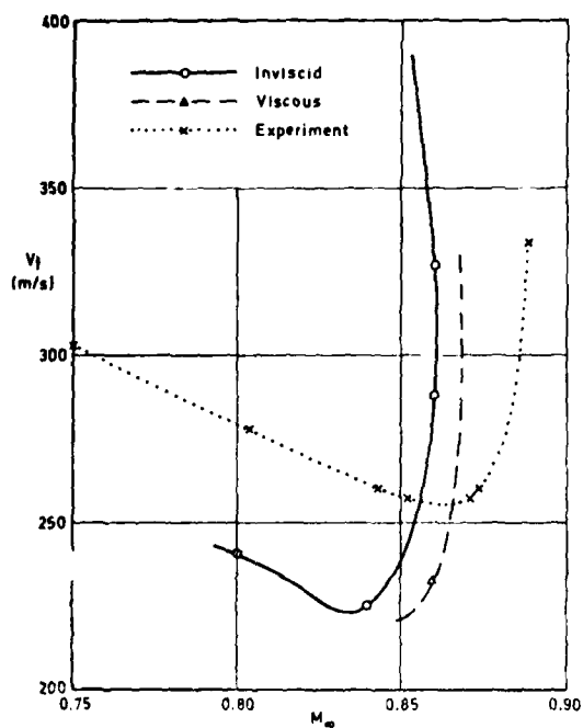
Fig 11 Flutter speeds predicted using strip-theory aerodynamics
