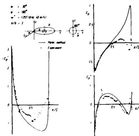
Figure 12: Ellipsoid of axis ratio a/b = 3 at \alpha = 30^\circ incidence. Steady and unsteady pressure distributions calculated by the present panel method compared with experimental results [14].
