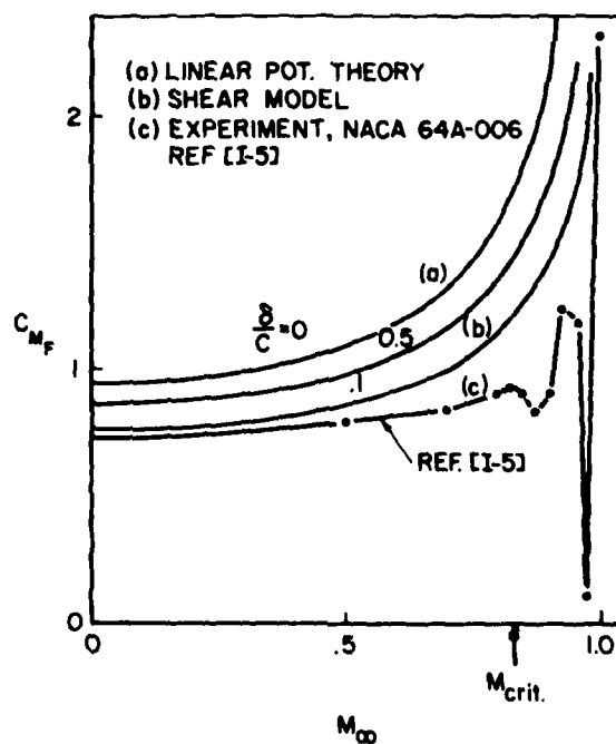
Fig.1-6 Static hinge moment, c_F/c .25
