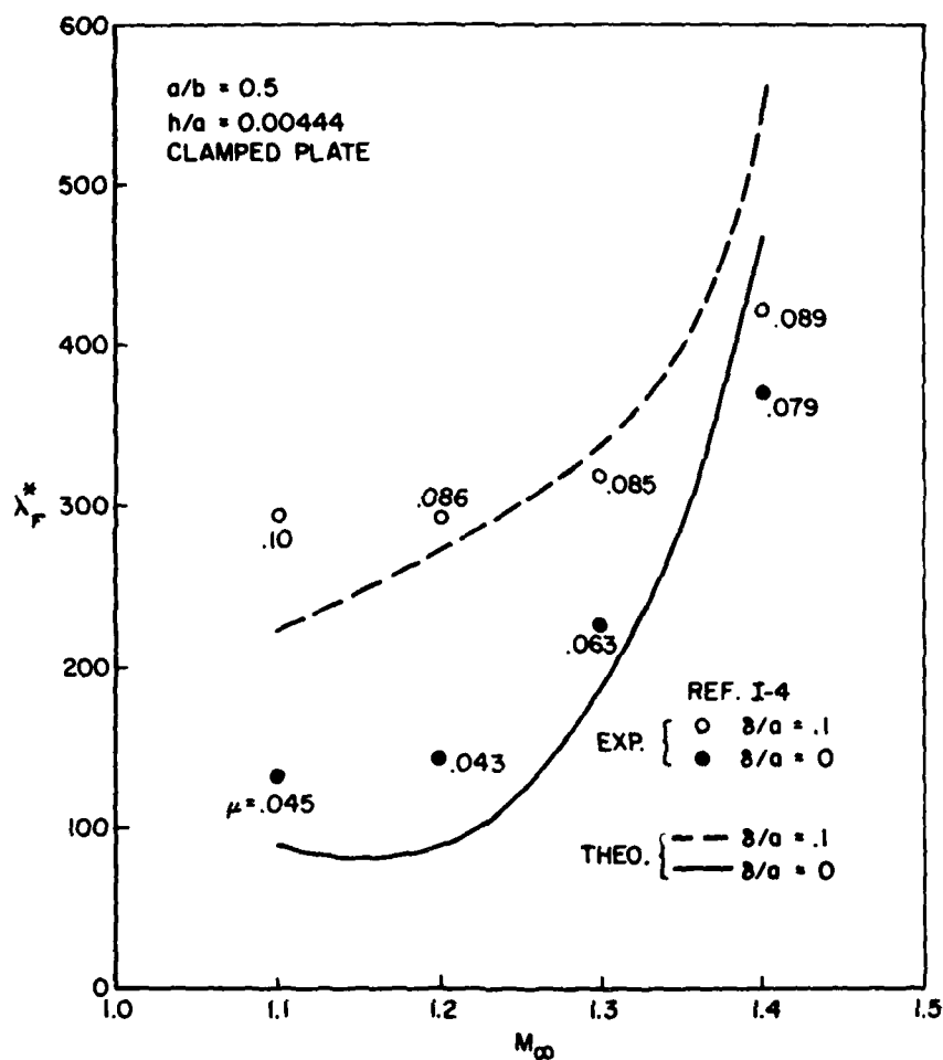
Fig.1-5 Panel flutter dynamic pressure vs. Mach number
