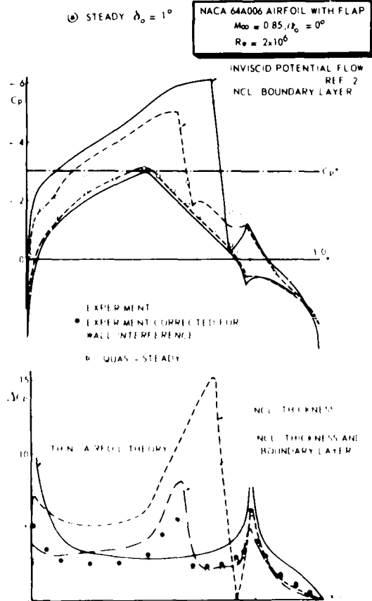
Fig. 3 Effect of boundary layer and unsteady airloads on the steady and quasi-steady airloads on the NACA 64A006 airfoil with flap at M_\infty = 0.85 , \delta_0 = 1^\circ
