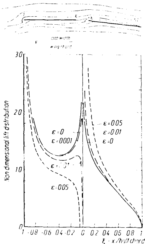
Figure 2: Effect of gap geometry on the unsteady pressures of wings with control surfaces performing translational oscillations. (Ref. [2])
