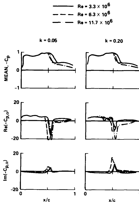
Fig. 7. Unsteady-pressure distribution on oscillating NLR 7301 airfoil; mean and first harmonic component, M = 0.807 , \alpha_m = 0.38^\circ , pitching \pm 0.5^\circ at 0.40 c .
