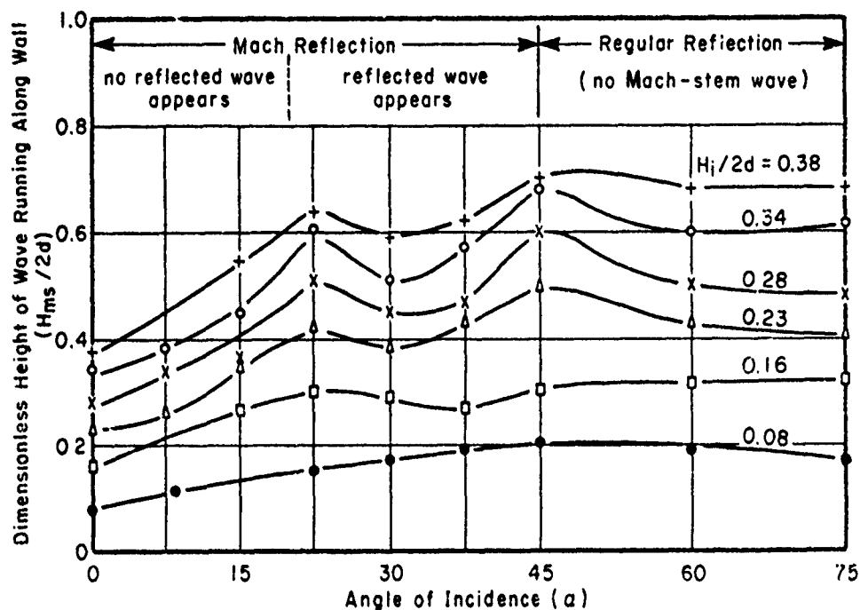
Figure 2. Oblique reflection of a solitary wave, experimental results; water depth, d = 0.132 foot (from Perroud, 1957).
