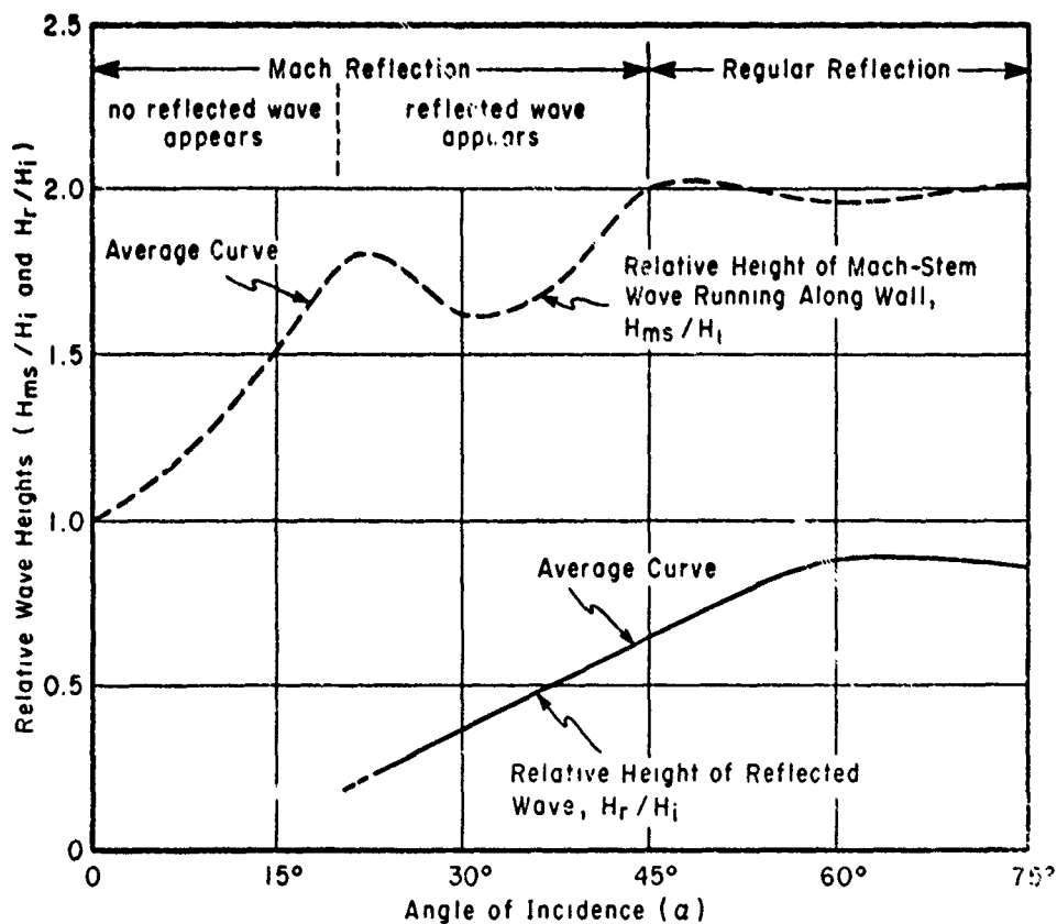
Figure 3. Oblique reflection of a solitary wave, experimental results (from Perroud, 1957).
