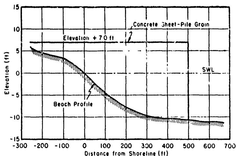
Figure 4. Beach and groin profile.
