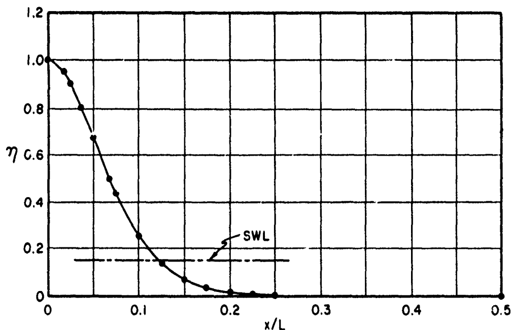
Figure 5. Dimensionless cnoidal wave profile, k^2 = 1 - 10^{-4.5} .
