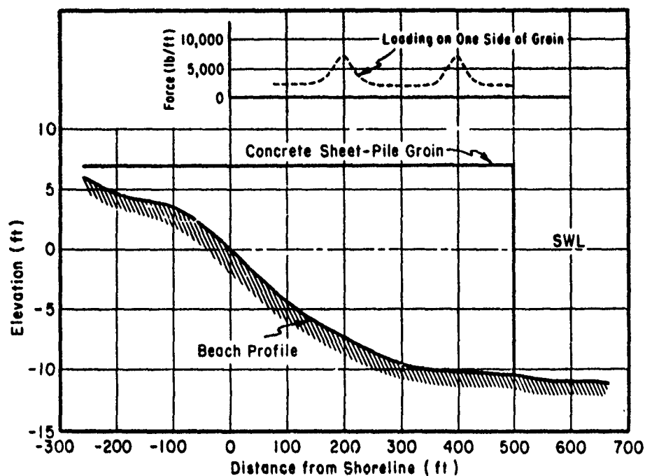
Figure 7. Loading on windward side of groin.
