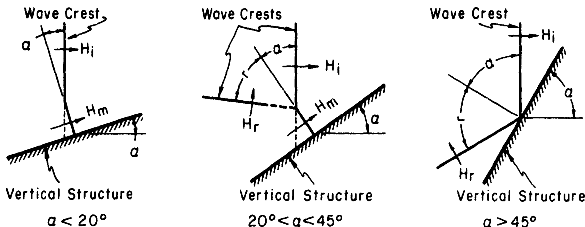
Figure 1. Reflection patterns of a solitary wave.
