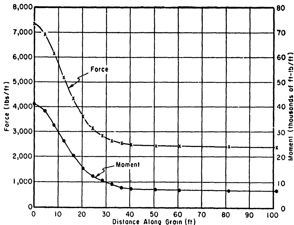
Figure 6. Variation of force and moment along groin.
