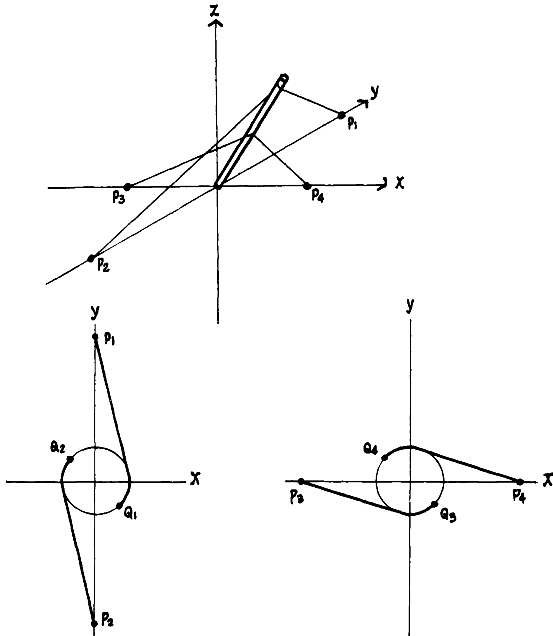
Figure 2-5. Schematic diagram of the arm showing the tendon wrapping geometry.
