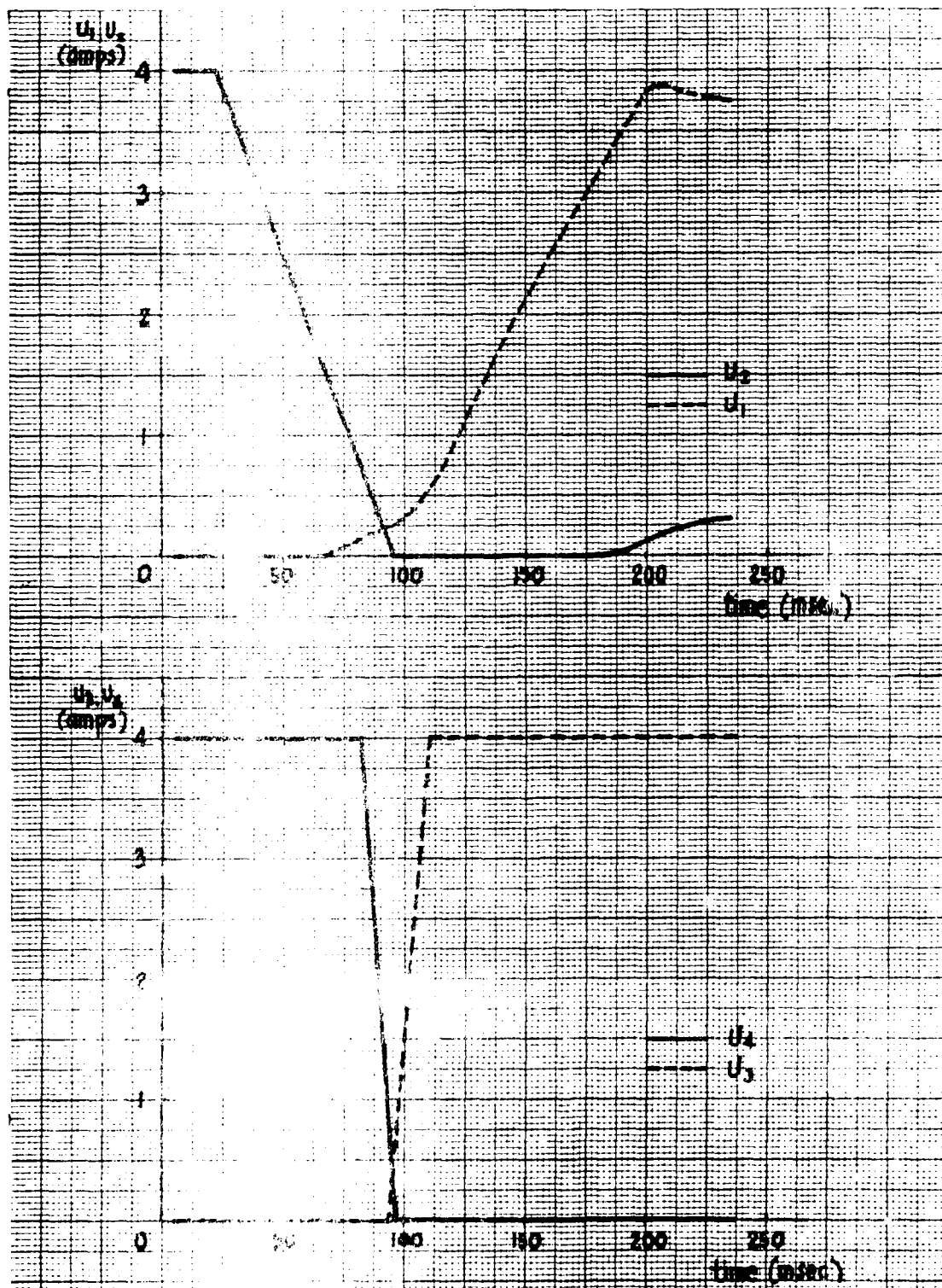
Figure 4-1. Current transients for \theta_f = 0.3614 , \phi_f = 0.3876 .
