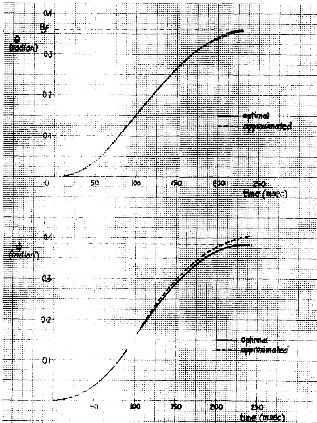
Figure 4.2. Comparison of the optimal and approximated control of figure 4.1 and 4.2
