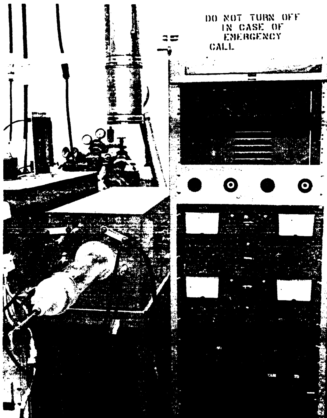
Fig. 78 Sulfurization Furnace
