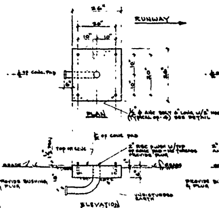
LIGHT CLUSTER MTG. PAD DETAIL NO SCALE
