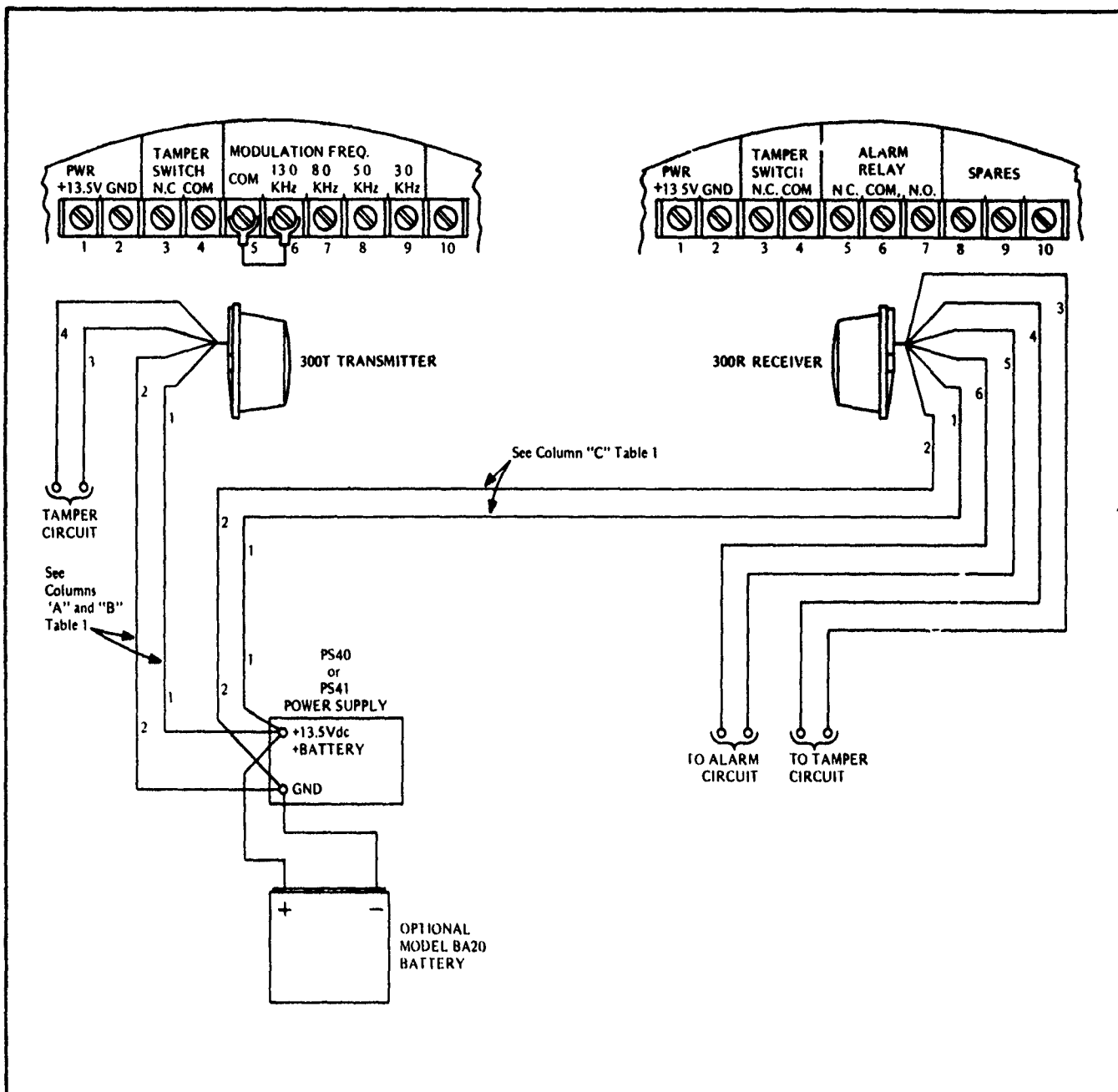
Figure 23 WIRING DIAGRAM
