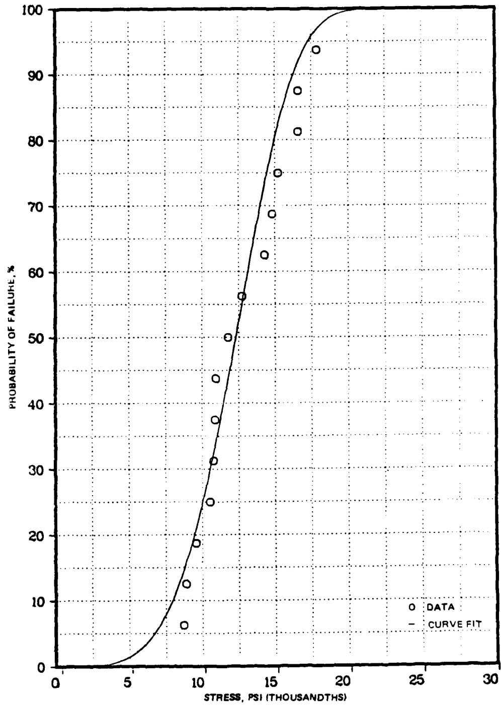
FIGURE 18. \text{MgF}_2 Equibiaxial Fracture Statistics ( T = 75^\circ\text{F} )
