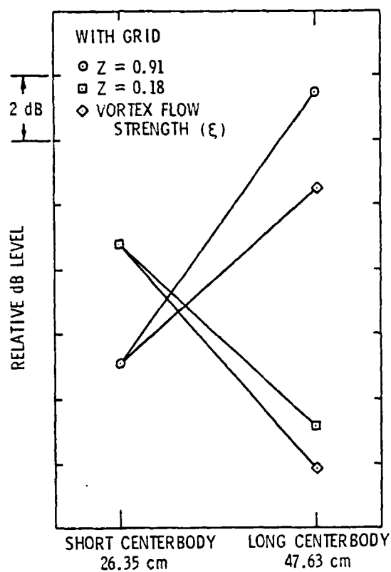
Figure 49. Comparison of Vortex Flow Strength to the First BPF, Grid Installed.
