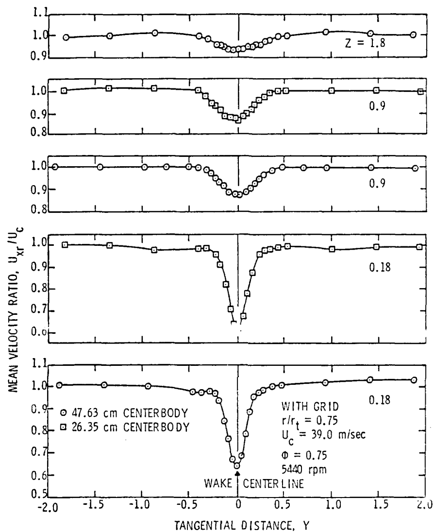
Figure 27. Mean Velocity Profiles at r/r_c = 0.75 as a Function of Rotor/Strut Spacing ( Z ), Grid Installed.
