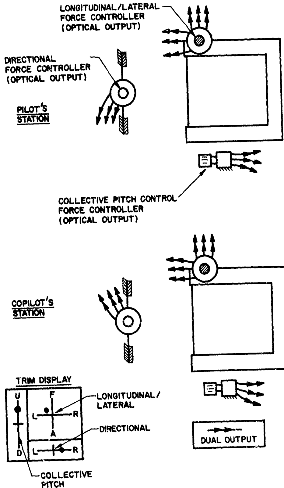
Figure A-1. Baseline Cockpit Control Concept.
