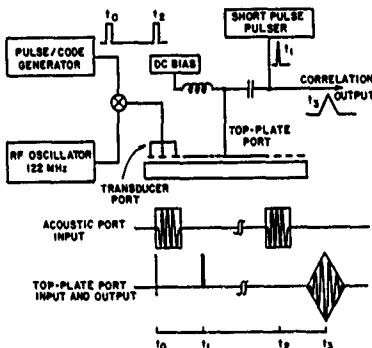
Figure 4 - Set up for acoustic to plate readout experiment t_1 = t_0 + 4 \mu\text{s} t_2 = t_0 + (20 \mu\text{s to storage time}) t_3 = t_2 + 4 \mu\text{s}
