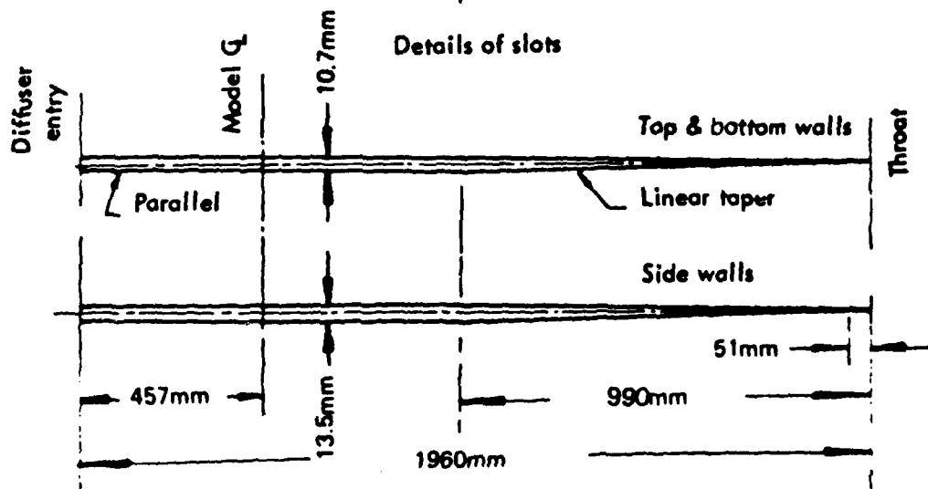
FIG. 4 DETAILS OF SLOTTED TEST SECTION
