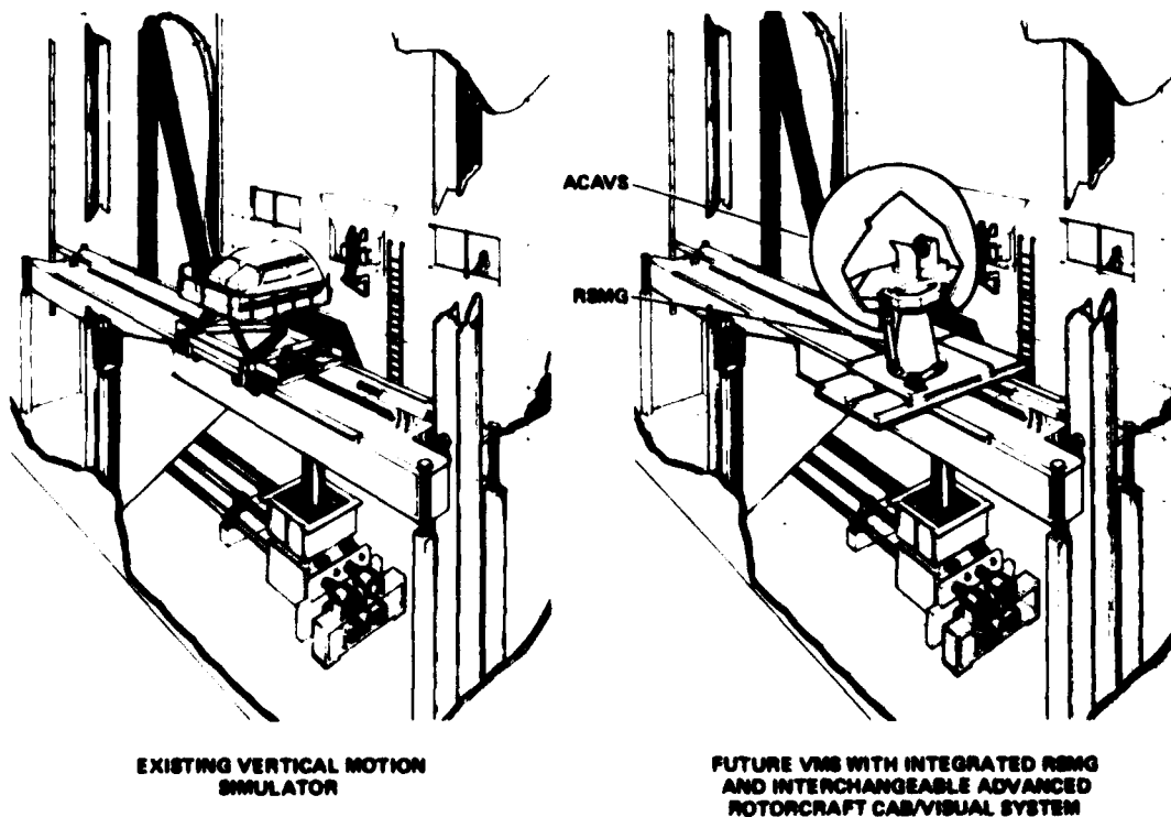
Fig. 14. Vertical Motion Simulator (VMS) RSIS project overview.
