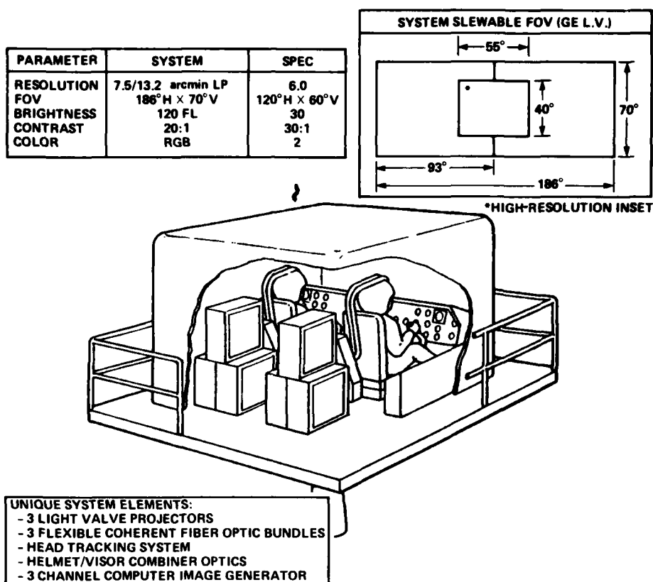
Fig. 19. Helmet-mounted display visual system concept.
