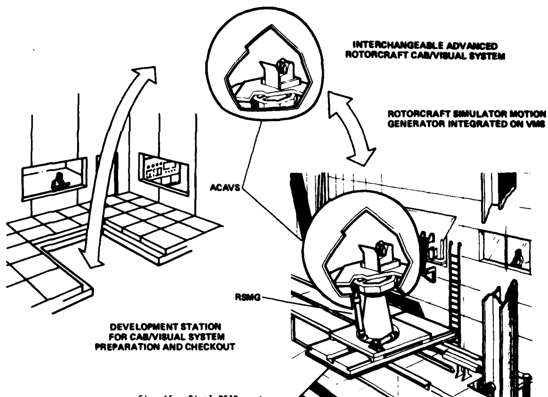
Fig. 15. Final RSIS system.
