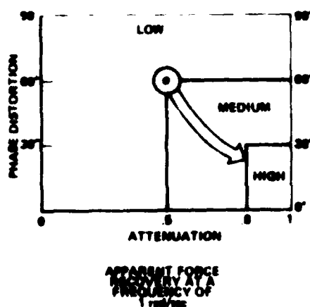
Fig. 9. Platform motion fidelity criteria.
