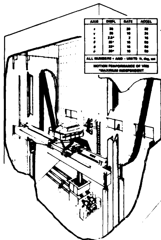
Fig. 13. Vertical Motion Simulator (VMS).
