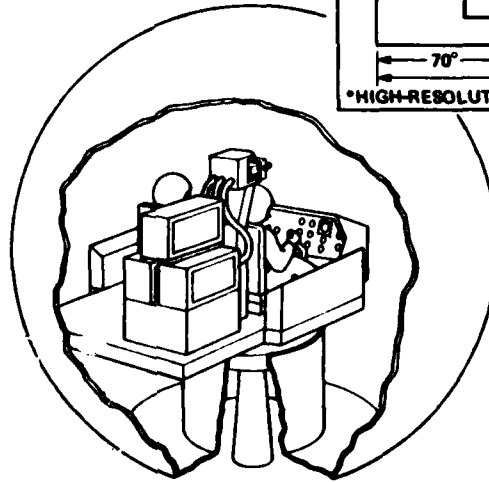
Fig. 17. Light-valve and fiber optics visual system concept.
