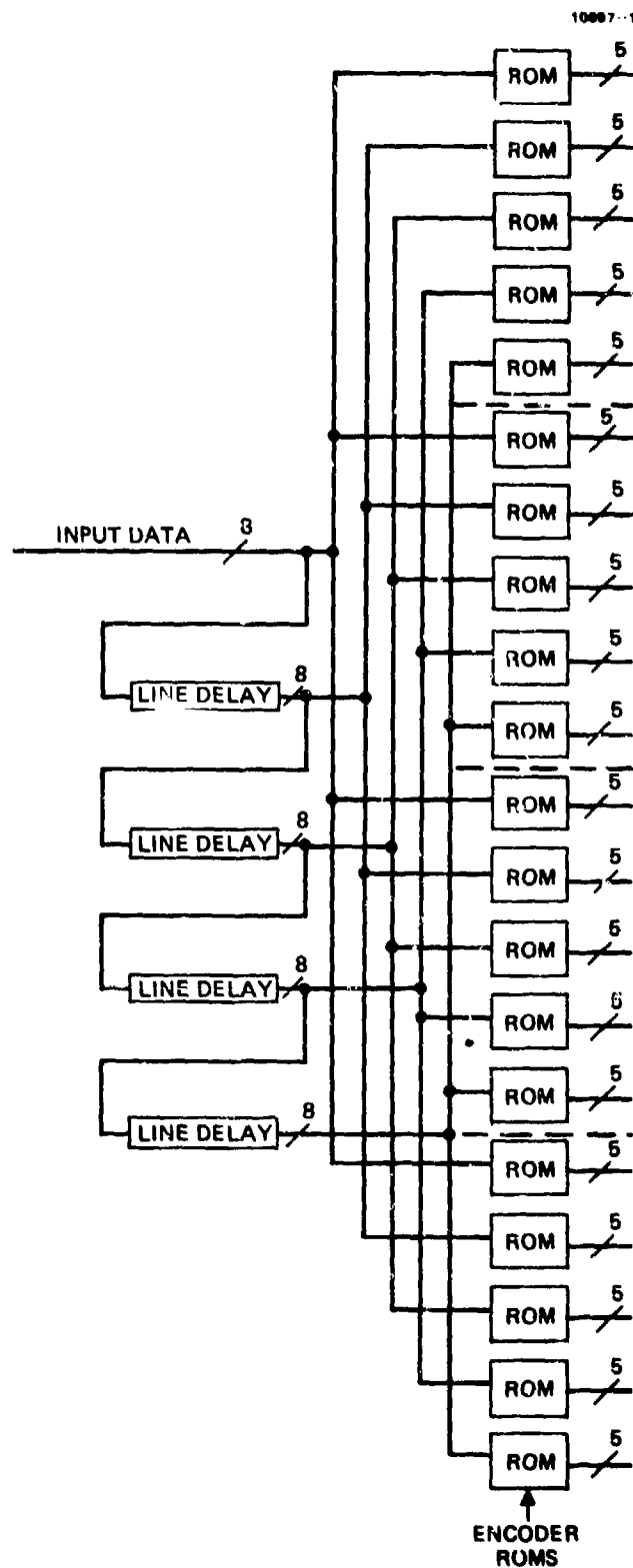
Figure 2. Kernel Generator Encoding for 5x5 Processor
