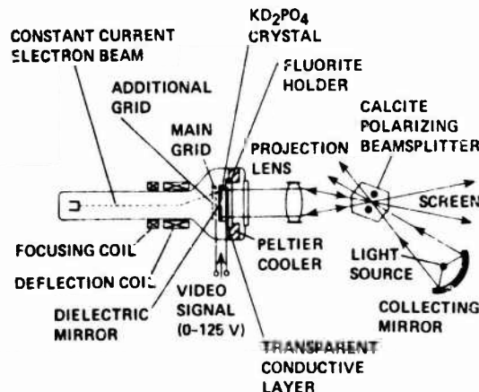
Fig. 62 Principle of operation, Titus tube-light valve projector
