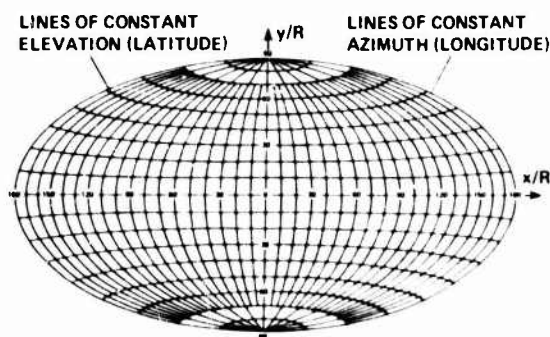
Fig. 65 Hammer's equal-area projection of a sphere
