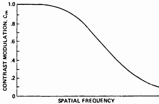
Fig. 32 Typical MTF curve
