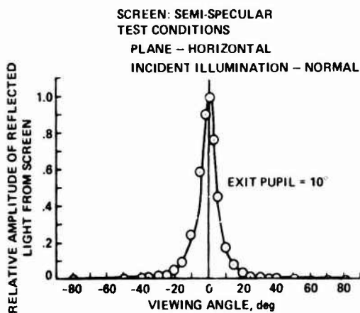
Fig. 50 Test data, semi-specular screen
