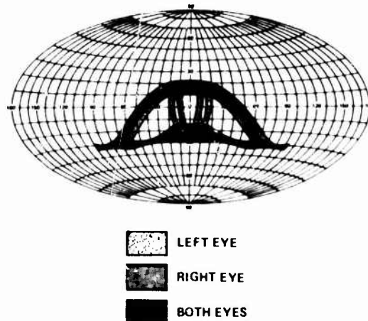
Fig. 66 Military strike aircraft (Panavia Tornado) binocular vision plot
