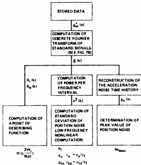
Fig. 75 Data analysis
