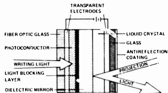
Fig. 61 LCLV fundamental functions
