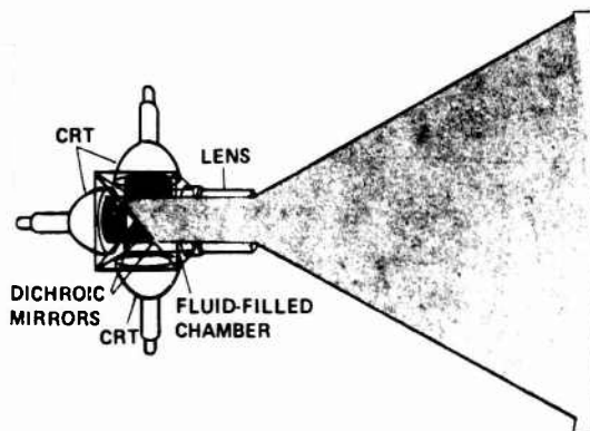
Fig. 59 Aquabeam color CRT projector
