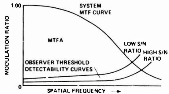
Fig. 45 Effect of noise on MTF
