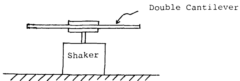
Figure 2 Damping of Cantilever Composite Plates
