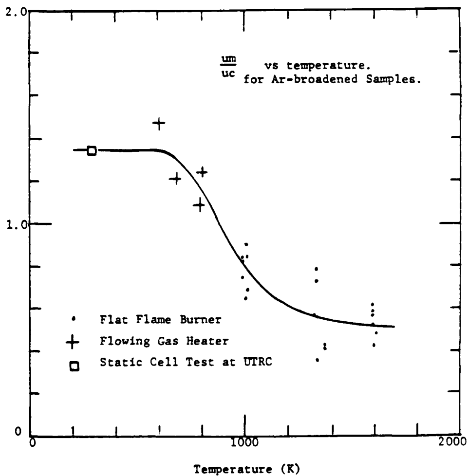
Figure 8. Plot of u_m/u_c vs Temperature for Ar-broadened samples.
