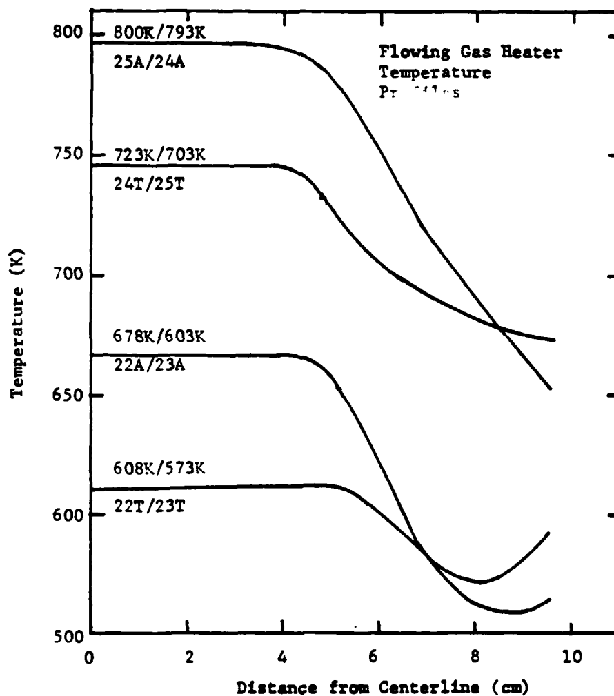
Figure 4. Temperature Profiles for the Flowing Gas Heater. The sample numbers for which the curves were used are written below each curve. The temperature at the center of the sample is listed above each curve.
