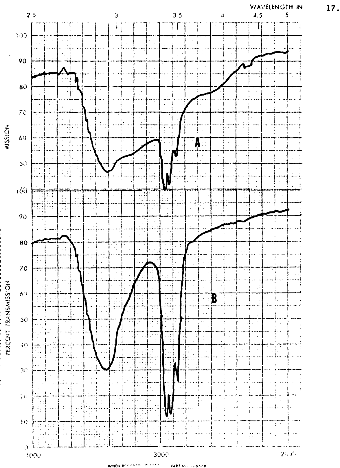
Figure 2. Comparison of the 4000 - 2000 \text{cm}^{-1} Infrared Spectral Region for Bicarbonate Soluble (A) and Bicarbonate Insoluble (B) Oligomeric Mixtures Derived by Treatment of the Ethyl Analogue with 1 N KOH for 5 Hours at 50° in the Presence and Absence of Oxygen Respectively.
