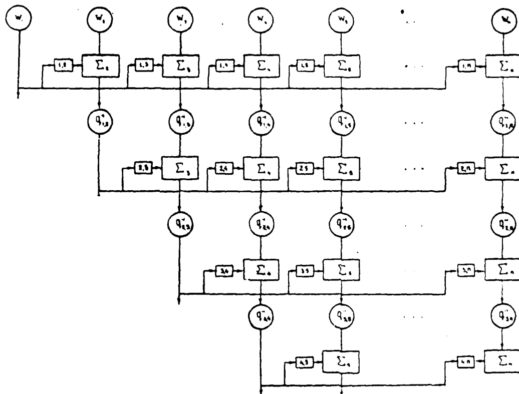
Fig. 44. Block diagram of translation algorithm ts.k.ch., preset by nonpositional code, into mixed positional code. \Sigma - adder, which realizes operation \langle x + iy \rangle_{q_k}^{\pm} .
