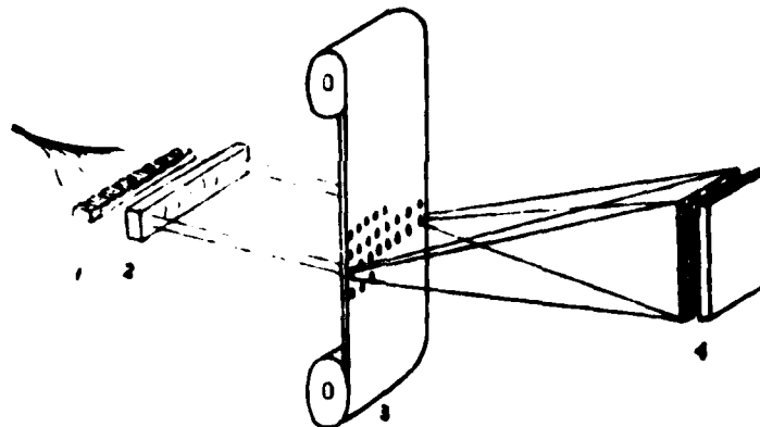
Fig. 12. Idealized diagram of enlarged holographic memory with a band of coupled lasers. 1 - laser band, 2 - deflector, 3 - tape with holograms, 4 - photodetector matrix.
