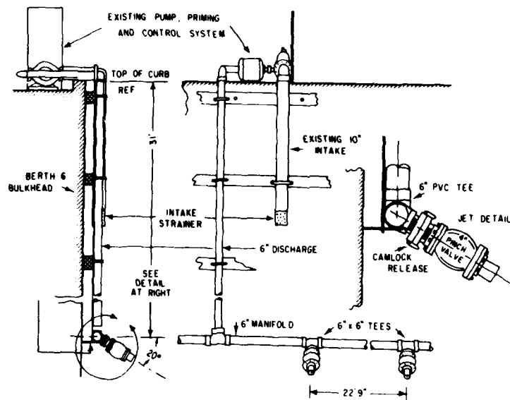
Figure 1-6. Quay Wall Installation of Water Jet Array
