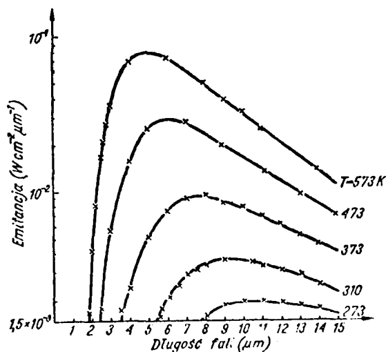
Figure 4. Spectral distribution of the emittance of back body at its various temperatures (310 K - temperature of human body). Ordinate: Emittance; abscissa: Wavelength.
