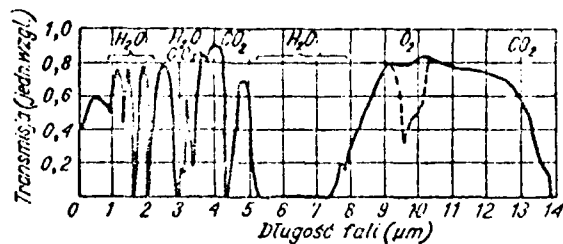
Figure 3. Spectral transmission of earth atmosphere at the distance 2000 m at sea level /3/. Ordinate: Transmission (arbitrary units); Abscissa: Wavelength
