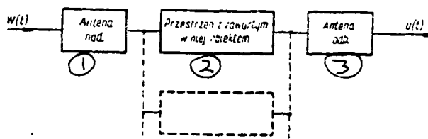
D.1.1. Substitute diagram of the system: transmitting antenna-space being scanned - receiving antenna. 1-transmitting antenna, 2-space with the object contained in it, 3-receiving antenna.
