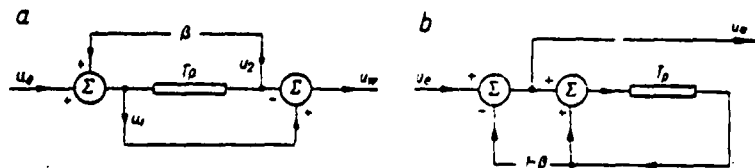
Fig. 8.1.9. Subtraction system with feedback.
