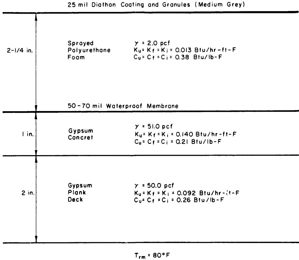
Figure 1. Roof System 5, Building 5, Cape Hatteras, NC.
