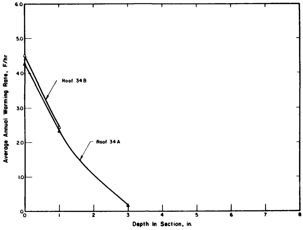
Figure 16. Average warming rates for roof systems on Building 34.
