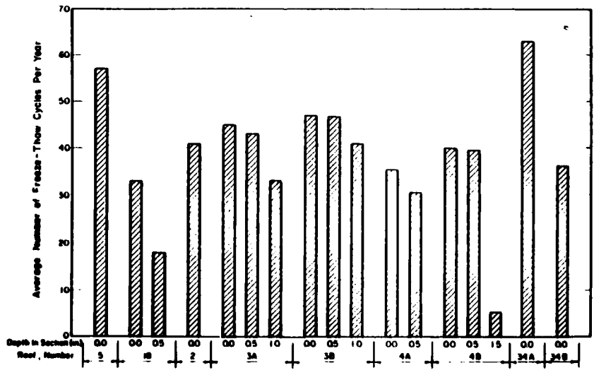
Figure 17. Average number of freeze-thaw cycles per year.
