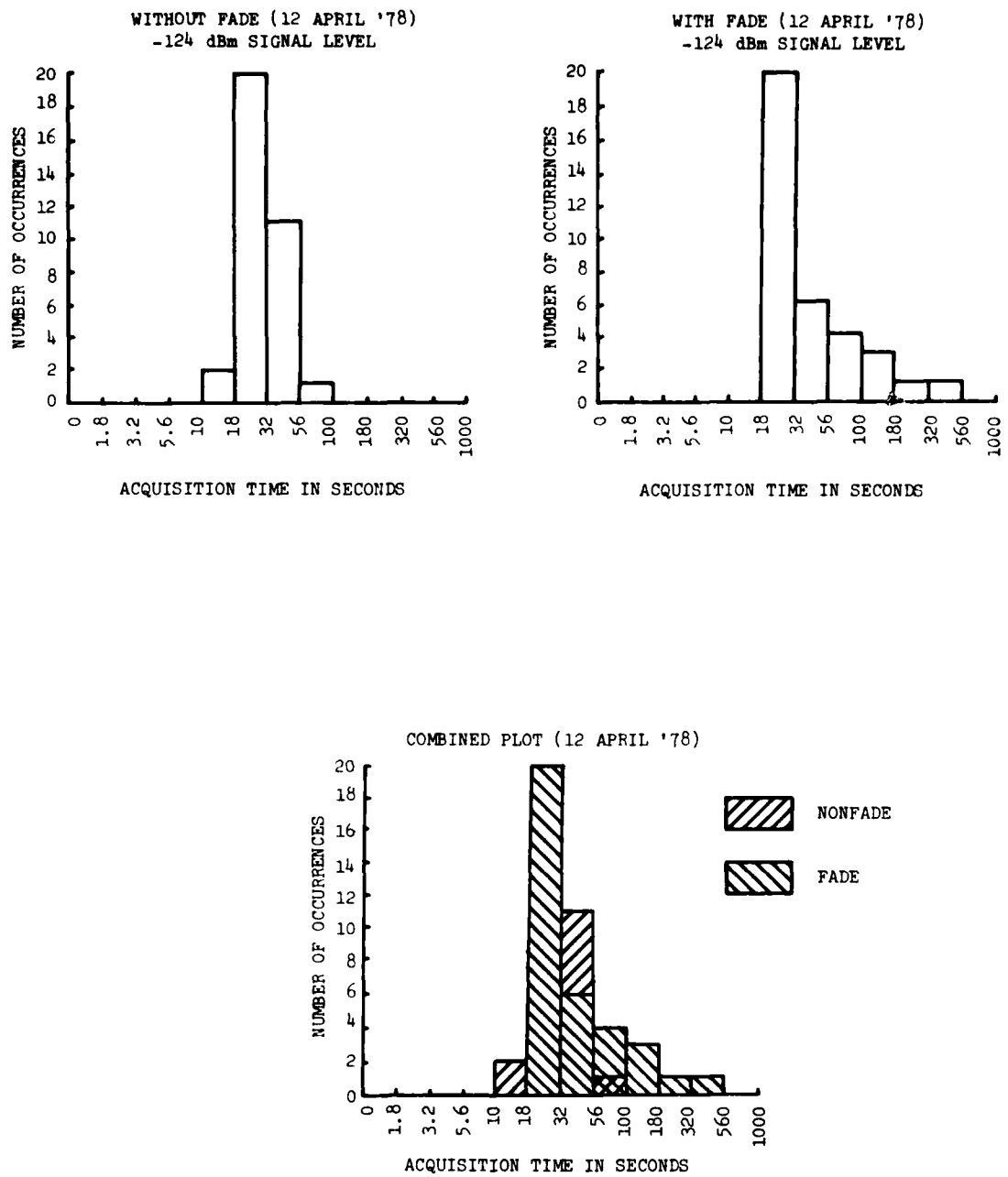
Figure 17. UHF Modem Acquisition Time
