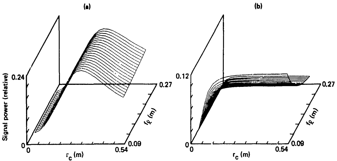
Figure 6. Laser heterodyne signal power results calculated by the stationary phase (a) and numerical integration technique (b) as a function of the local oscillator focal length, r_Q , and Schell-model coherence length, r_c . Fixed parameters of the calculation are A = 2 mm, P = 2.5 cm, L_o = 8 cm, f_r = 25 cm, L_\phi = -200 m, and R = 200 m.
