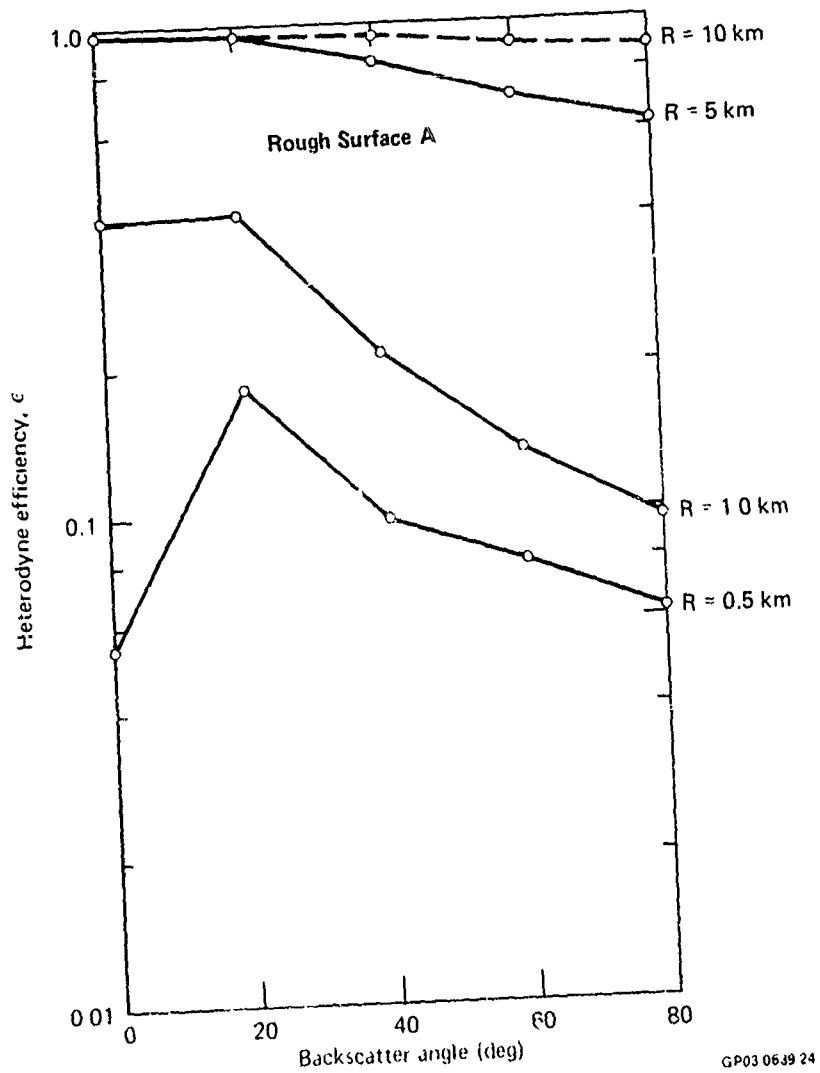
Figure 24. Laser heterodyne detection efficiency values computed as a function of view-in (backscatter) angle for a conical target having a base radius of 0.25 m, a height of 1.0 m, and a surface finish characterized by rough surface A. Fixed parameters of the calculation are A = P = 2.5 cm, f_t = f_r = 25 cm, L_o = 5 cm, C_n^2 = 10^{-14} \text{ m}^{-2/3} , and range (R) values are annotated.
