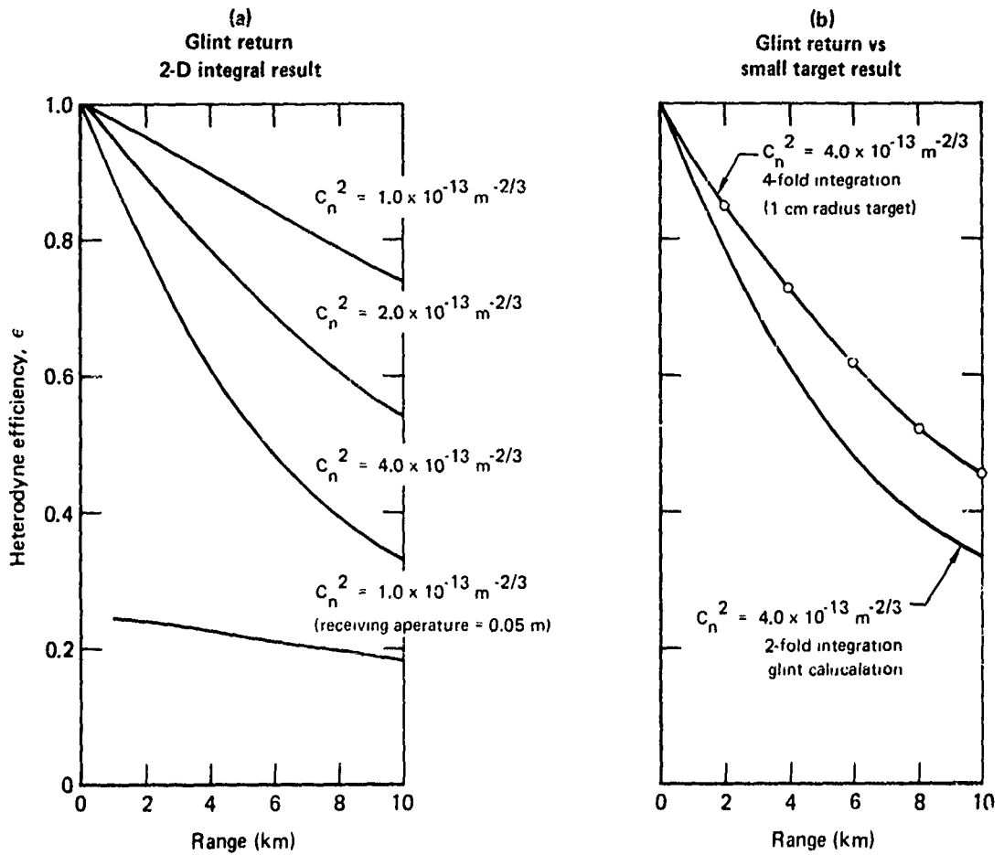
Figure 16. Laser heterodyne maximum detection efficiency computed as a function of range for (a) a single target glint using the two-fold integral Schell-model method and (b) a 1 cm radius target (having a Gaussian intensity distribution) using the approximate four-fold integral method. Fixed parameters of the calculation are A = P = 2.5 cm, f_Q = f_r = 25 cm, and L_0 = 5 cm.
