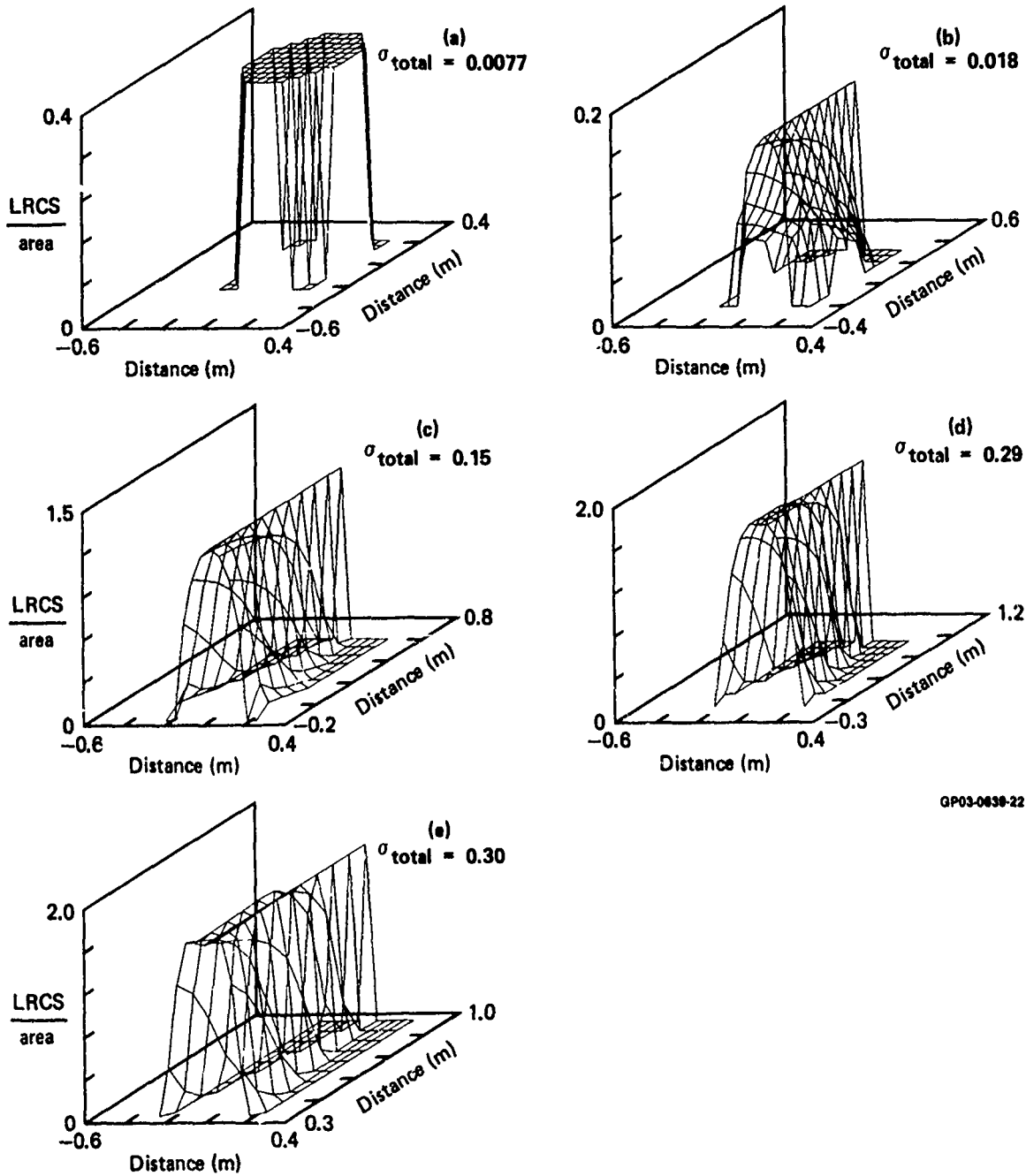
Figure 22. Projected laser cross section per unit area distributions for a conical target having a base radius of 0.25 m, a height of 1.0 m, and a surface finish characterized by rough surface B. Projection direction angles are (a) 0^\circ , (b) 20^\circ , (c) 40^\circ , (d) 60^\circ , and (e) 80^\circ .
