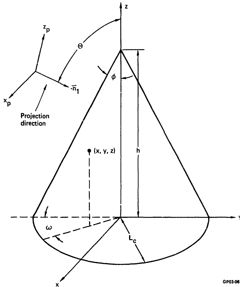
Figure 3. Cone projection geometry.
