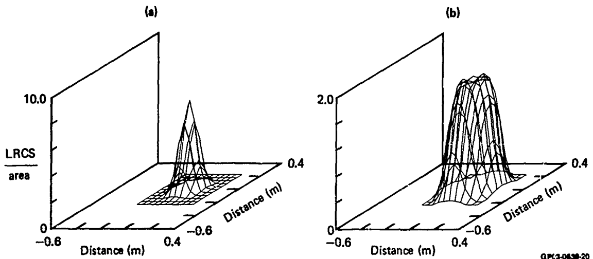
Figure 20. Projected laser cross section per unit area distributions for spherical targets (0.25 m radius) having surface characteristics of (a) rough surface A and (b) rough surface B.
