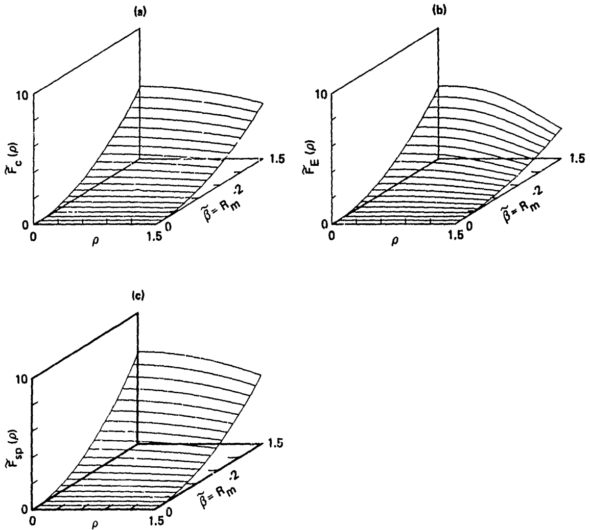
Figure 13. Laser radar filter function calculated by (a) numerical integration, (b) series expansion, and (c) stationary phase approximation as a function of the unitless variable \rho = R_m \mu' and the parameter \tilde{\beta} = R_m^{-2} .
