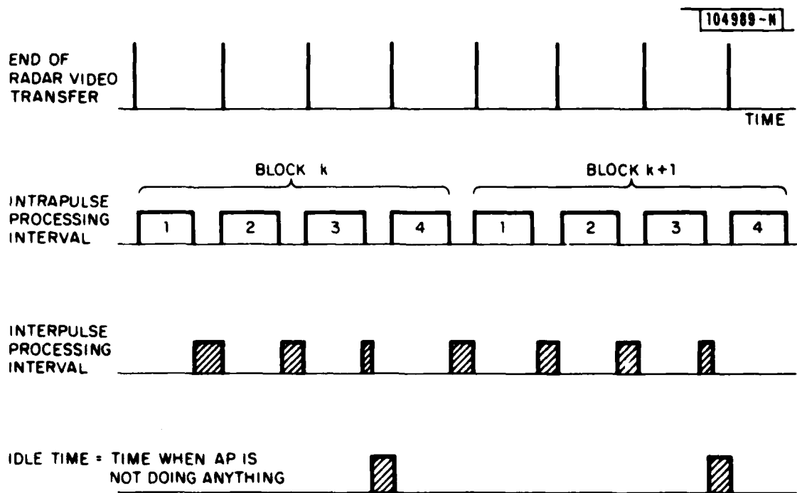
Fig. 3. Timing sequence.
