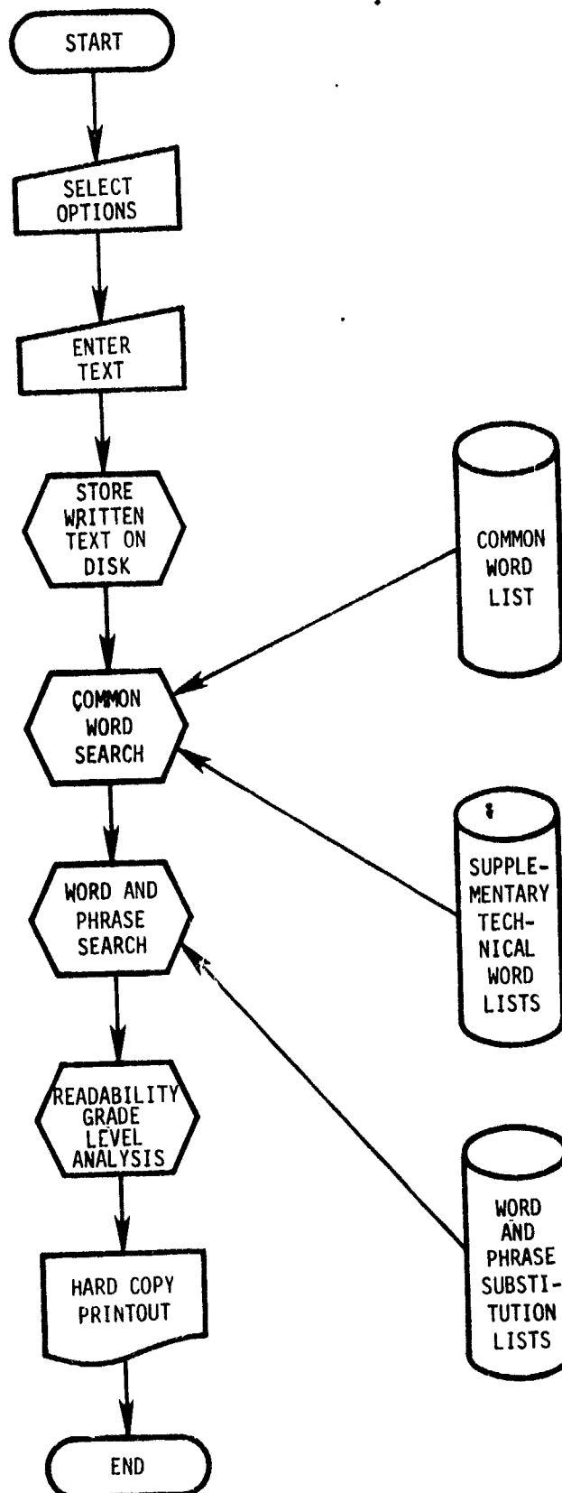
Figure 1. Flow Chart Showing Phases of Editing by the Computer Readability Editing System
