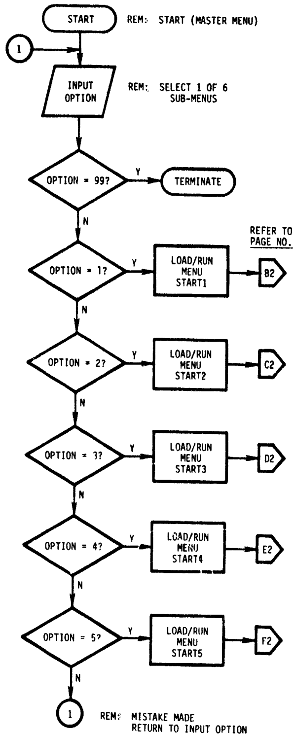
Figure 6. Flow Chart For Master Menu
