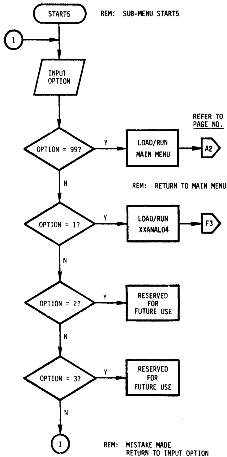
Figure 11. Flow Chart For the Text Analysis Subsystem
