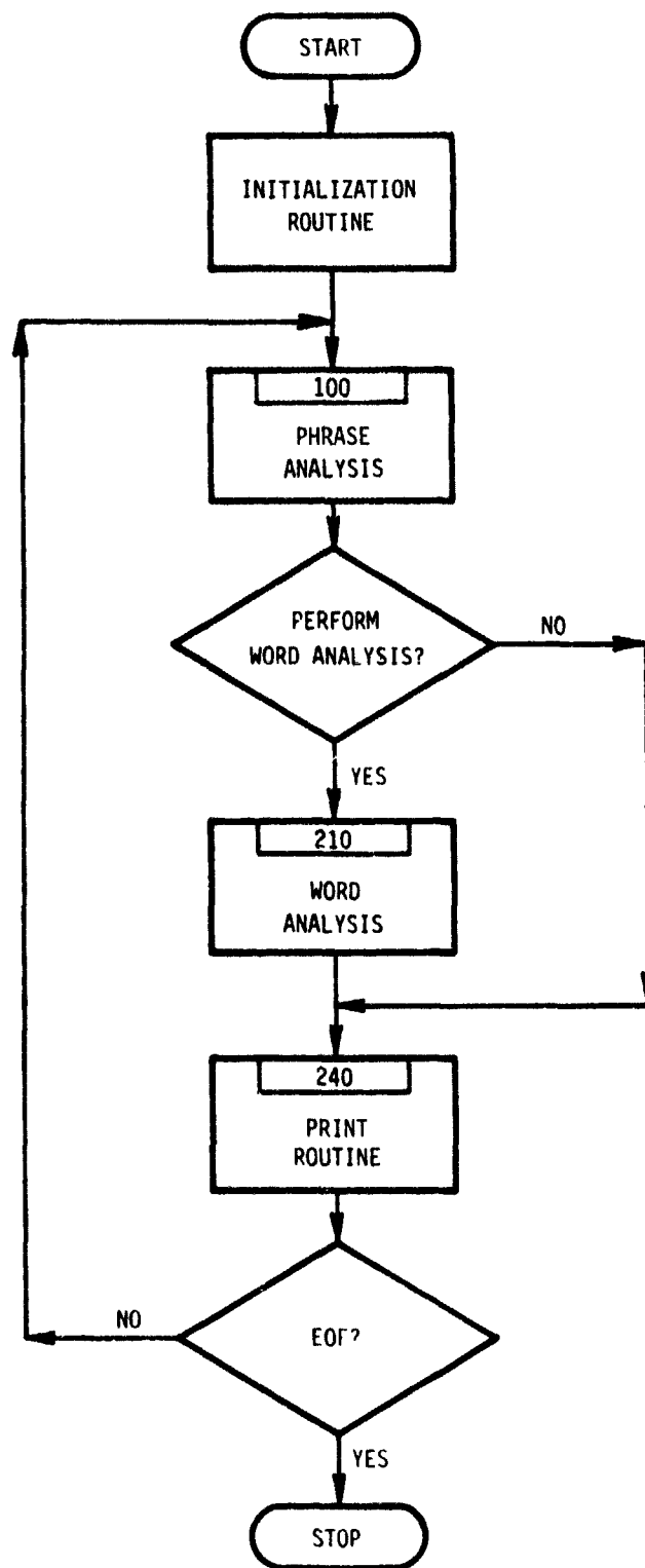
Figure 12. Flow Chart For Program XXANAL04
