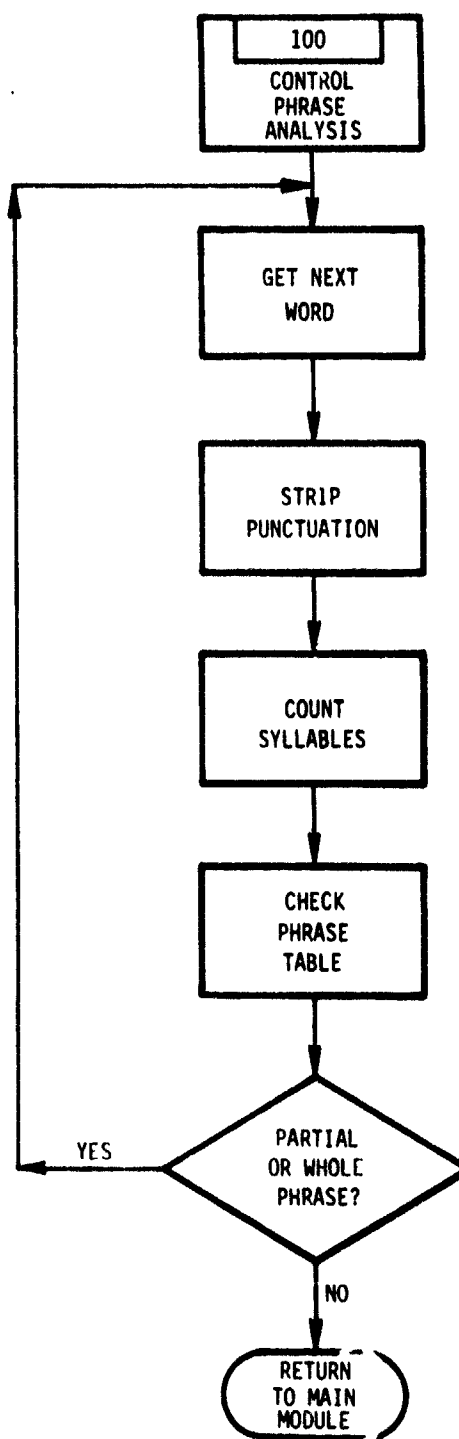
Figure 13. Flow Chart for The Phrase Analysis Subroutine of XXANAL04
