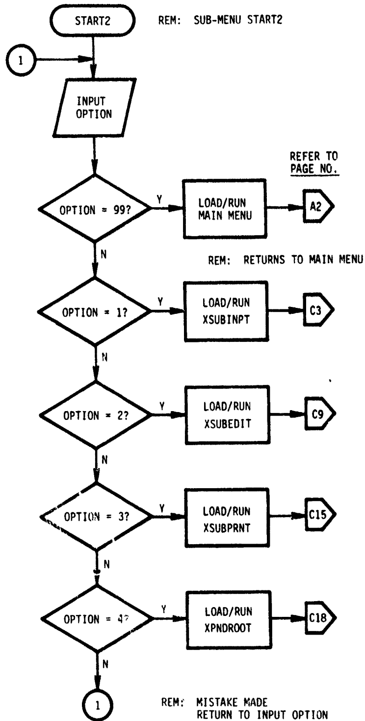
Figure 8. Flow Chart For Word Substitution File Subsystem Menu
