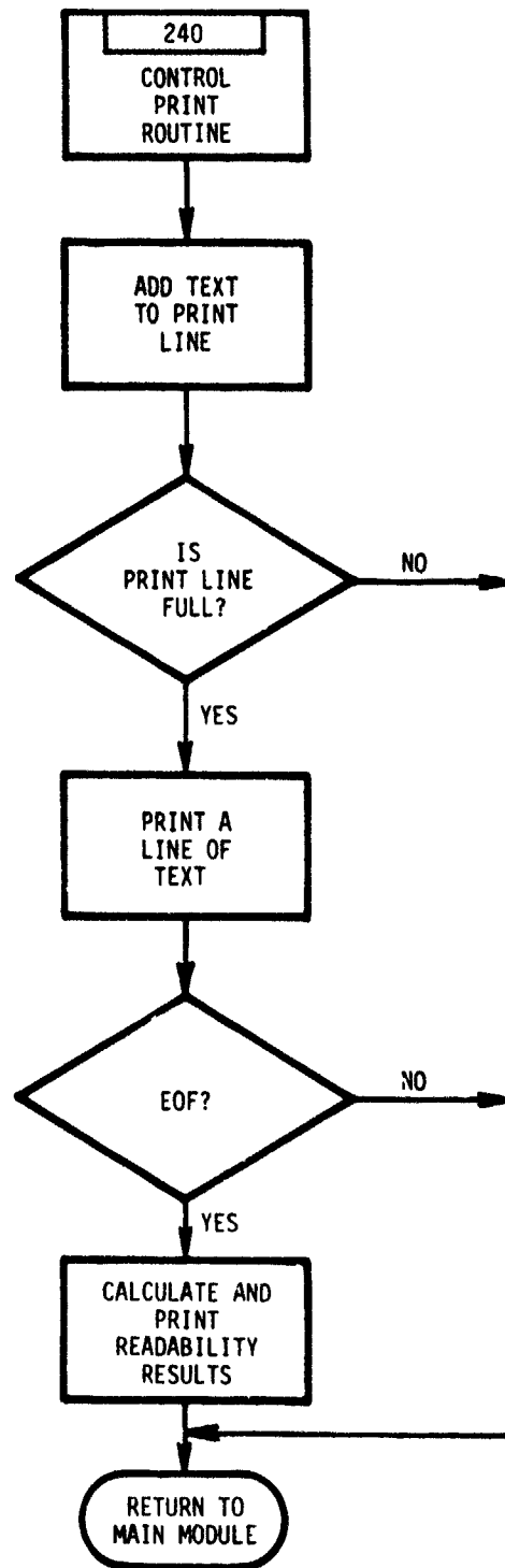
Figure 15. Flow Chart For The Print Subroutine of XXANAL04
