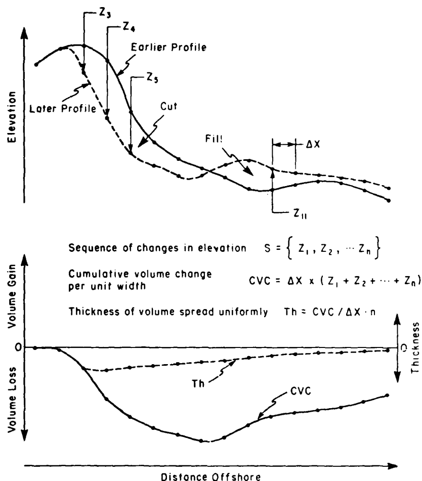
Figure 12. Schematic diagram of volume change calculations.
