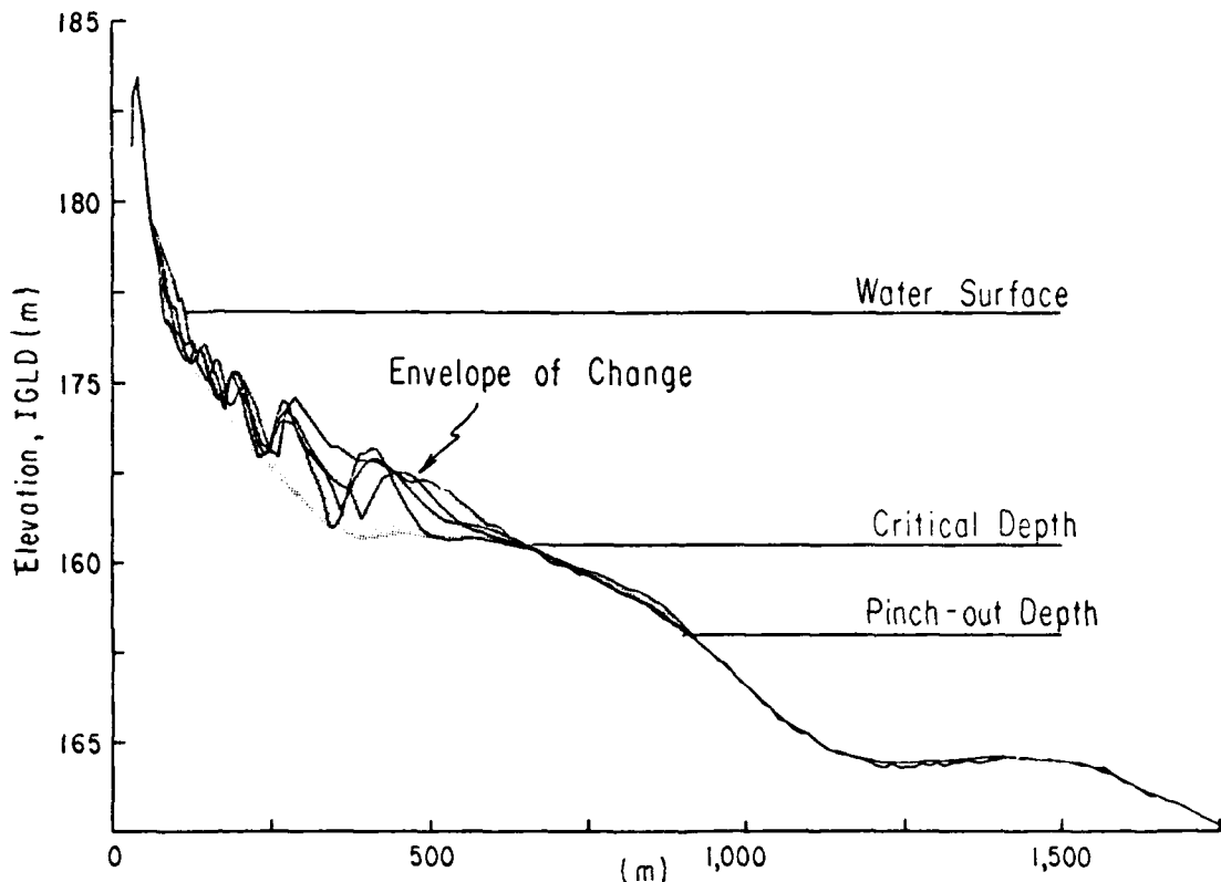
Figure 10. Envelope of bottom change, station 4 (1967-75). After several years of profile adjustment to higher water levels, the envelope of changes in bottom elevation is thickest in the zone traversed by the largest migrating bar and narrows abruptly above the wave uprush and below the barred zone.
