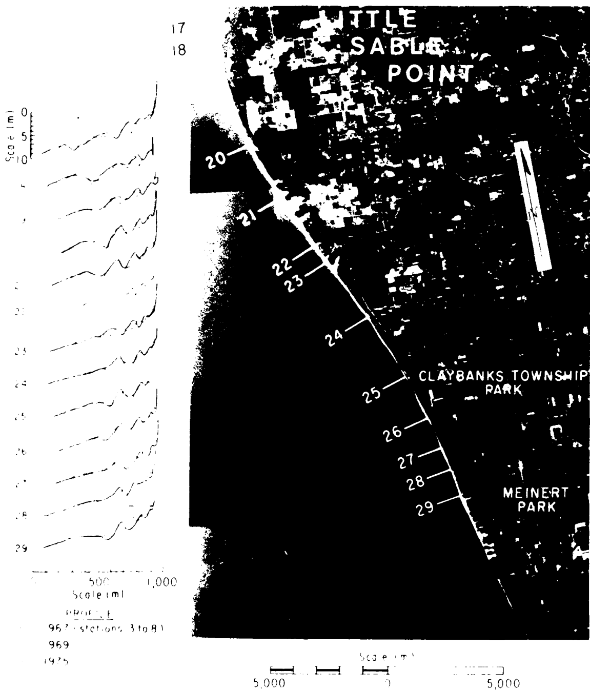
Figure 10. Wet results of long-term infiltration. Changes in bathymetry and mean water levels are shown by profiles for the 1967, 1969, and 1975 conditions. Profile stations are arranged by order from northernmost station 1 to southernmost station 29.—continued
