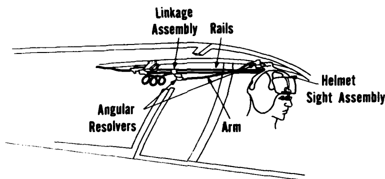
FIGURE 2. Mechanical linkage.
