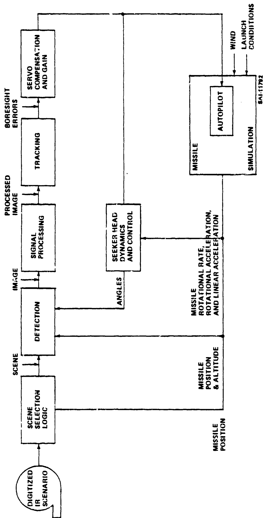
Figure 1-2. TGSM System with Target Imaging Generator Using HELLFIRE Math Modeling Where Applicable
