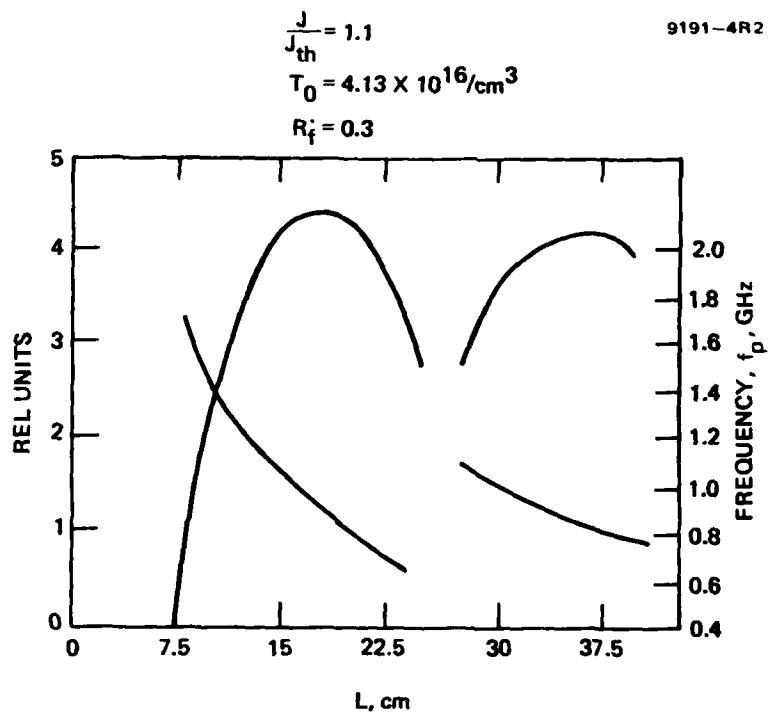
Figure 22. Calculated plot showing the variation of induced pulse amplitude versus external cavity length.
