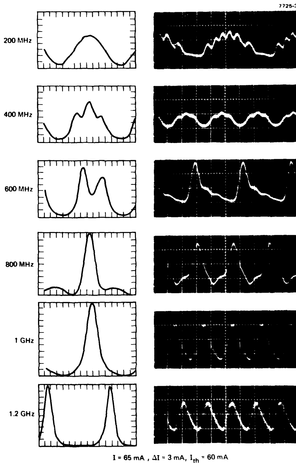
Figure 6. Large-signal modulation of injection lasers output optical waveforms for sinusoidal current variations.
