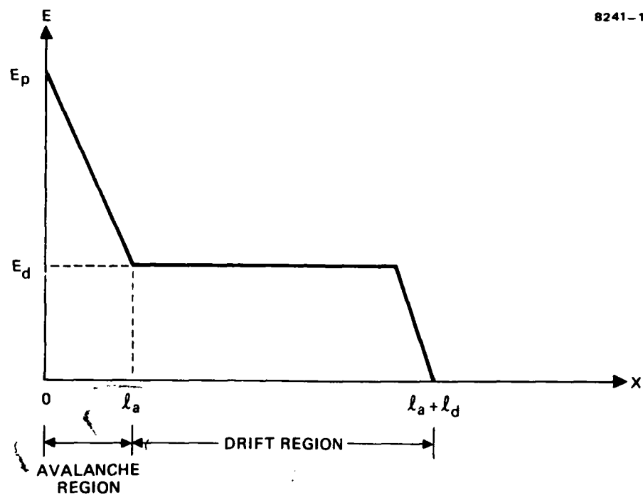
Figure 6. Electric field distribution inside an IMPATT diode.
