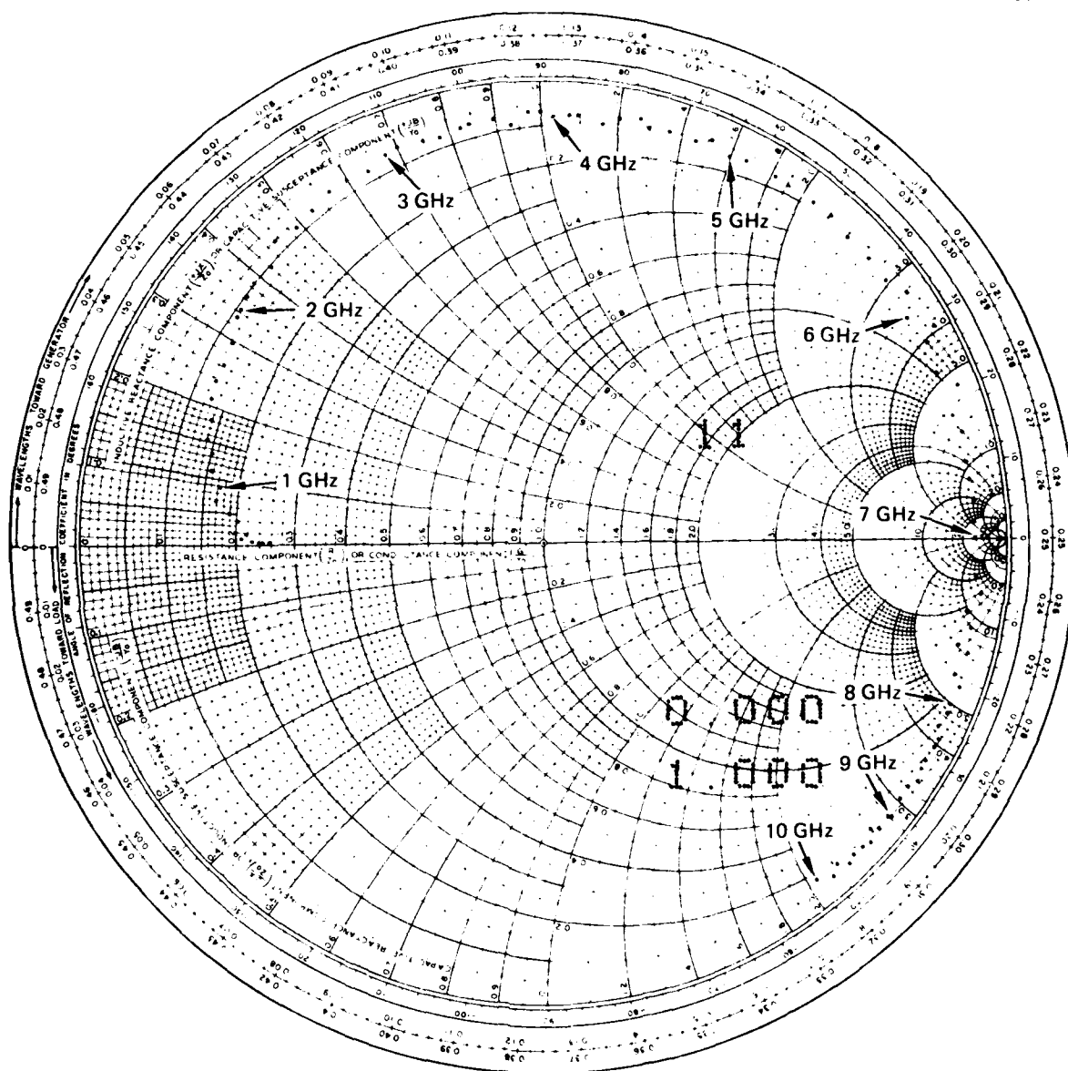
Figure 11. Hitachi BH laser (HLP 2400U) impedance from 100 MHz to 10 GHz in 100-MHz steps. Smith chart is normalized to 50 \Omega .
