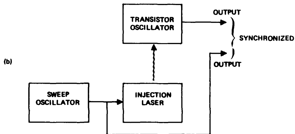
Figure 14. Schematics of two optical injection locking schemes.
