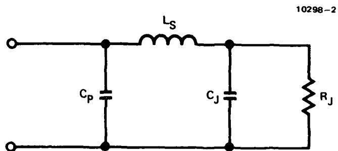
Figure 10. Equivalent circuit of the (GaAl)As injection laser.
