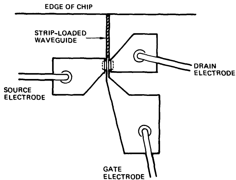
Figure 49. Top view of the waveguide FET detector. The dimensions of the MESFET are: width is 50 \mu\text{m} , length is 50 \mu\text{m} , source-drain spacing is 10-15 \mu\text{m} , gate length is 5 \mu\text{m} .
