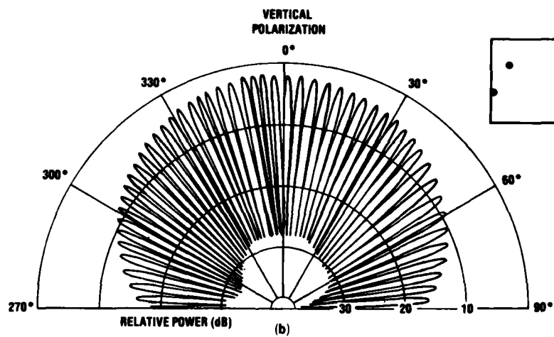
Figure 6. Typical spin-linear radiation patterns of 6.2-cm square patch in horizontal and vertical polarized configurations. Substrate and ground plane are 22 cm square.
