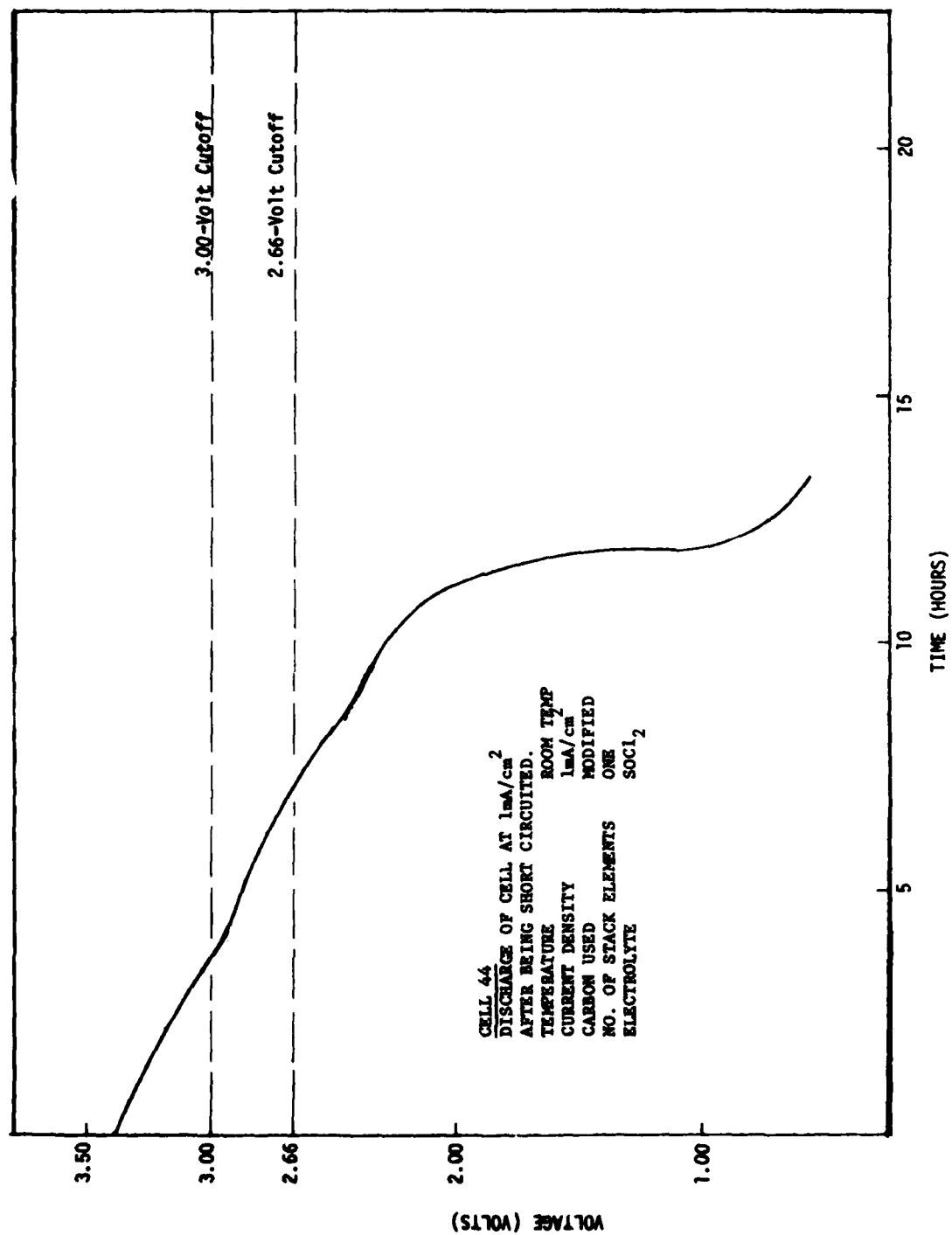
Figure 50. Discharge Results - Disc Cell 44
