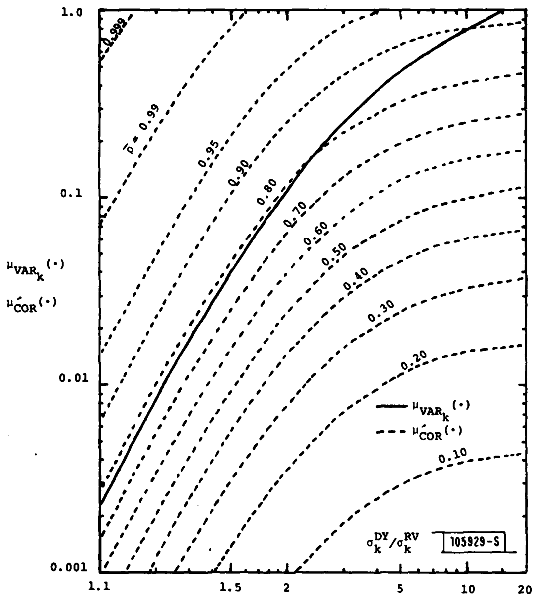
Fig. 2. Variation of Bhattacharyya distances due to variance differences in band k , with \mu_{\text{COR}}^{(\cdot)} shown for several values of average band-to-band correlation.
