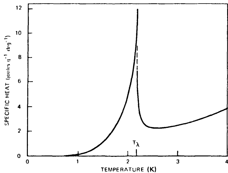
Figure 3-2. The specific heat of liquid He 4 in the neighborhood of the λ point transition.
