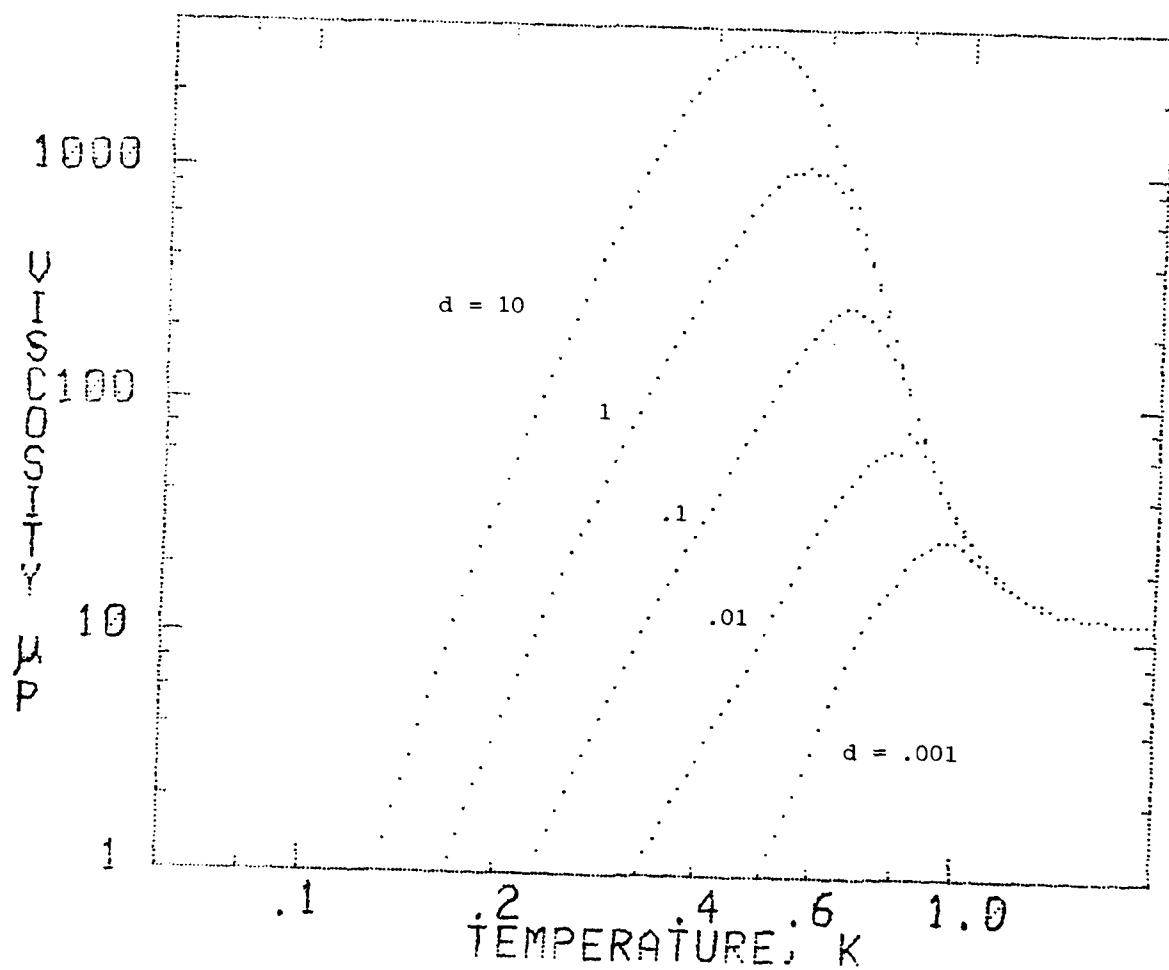
Figure 3-15. The theoretical effective viscosity of liquid \text{He}^4 for various fluid gaps d in cm, with \gamma_1 = \gamma_2 = .4 , \delta_1 = \delta_2 = 100\text{\AA} and X_3 = 10^{-12} .
