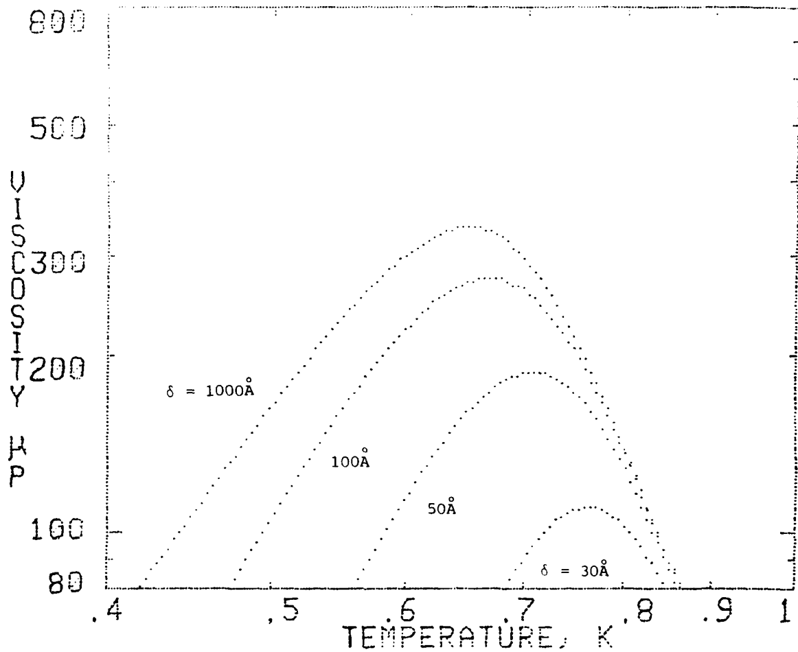
Figure 3-17b. The theoretical effective viscosity of liquid He 4 for various surface roughness factors \delta , with d = .1 cm, \gamma_1 = .3 , \gamma_2 = .6 , \delta_1 = \delta , \delta_2 = 1000\text{\AA} and x_3 = 10^{-12} .
