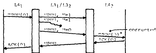
Fig. 2.5: Error situation with fragmentation of transport-ndus
