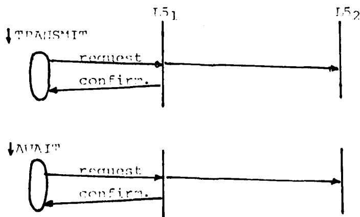
Fig. 5.4: Message exchange
