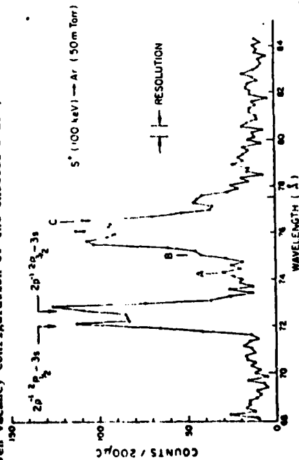
Figure 1. Portion of the grazing-incidence spectrum from 100 keV S^{+} - Ar collisions. The 68-84 Å region shown has mostly neonlike and sodiumlike sulfur L-M X-ray transitions (range 182-148 eV). The doublet identified arises from neonlike S^{6+} 1s^2 2s^2 2p^1 \frac{1}{2}, \frac{3}{2} 3s fine-structure states, with \omega_L = 1 and wavelengths 72.029 and 72.663 Å. Transitions A, B, C, having fluorescence yields less than 12, are discussed in the text.
