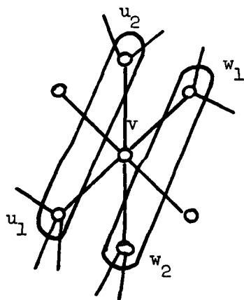
Figure 5. Deletion and contraction near vertices in S .
