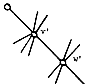
Figure 5. Deletion and contraction near vertices in S .
