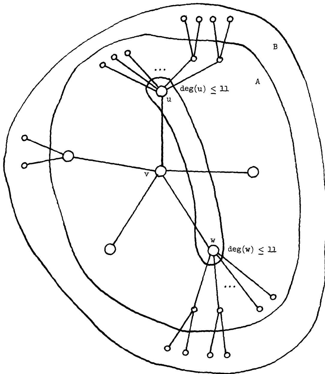
Figure 2. Deletion and contraction step. Vertices in region A will have their adjacency lists updated. Vertices shown in B have degree five and need to be placed in appropriate 5^{[11]} - or 5-degree lists.
