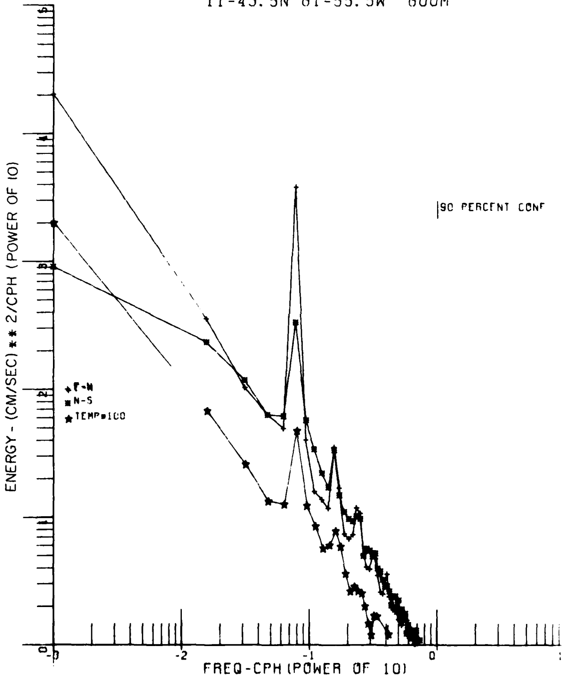
Figure 21. Variance spectra of flow components and temperature ( T^2/cph ) at in Grenada Passage (see Table 1). Data were not filtered.
