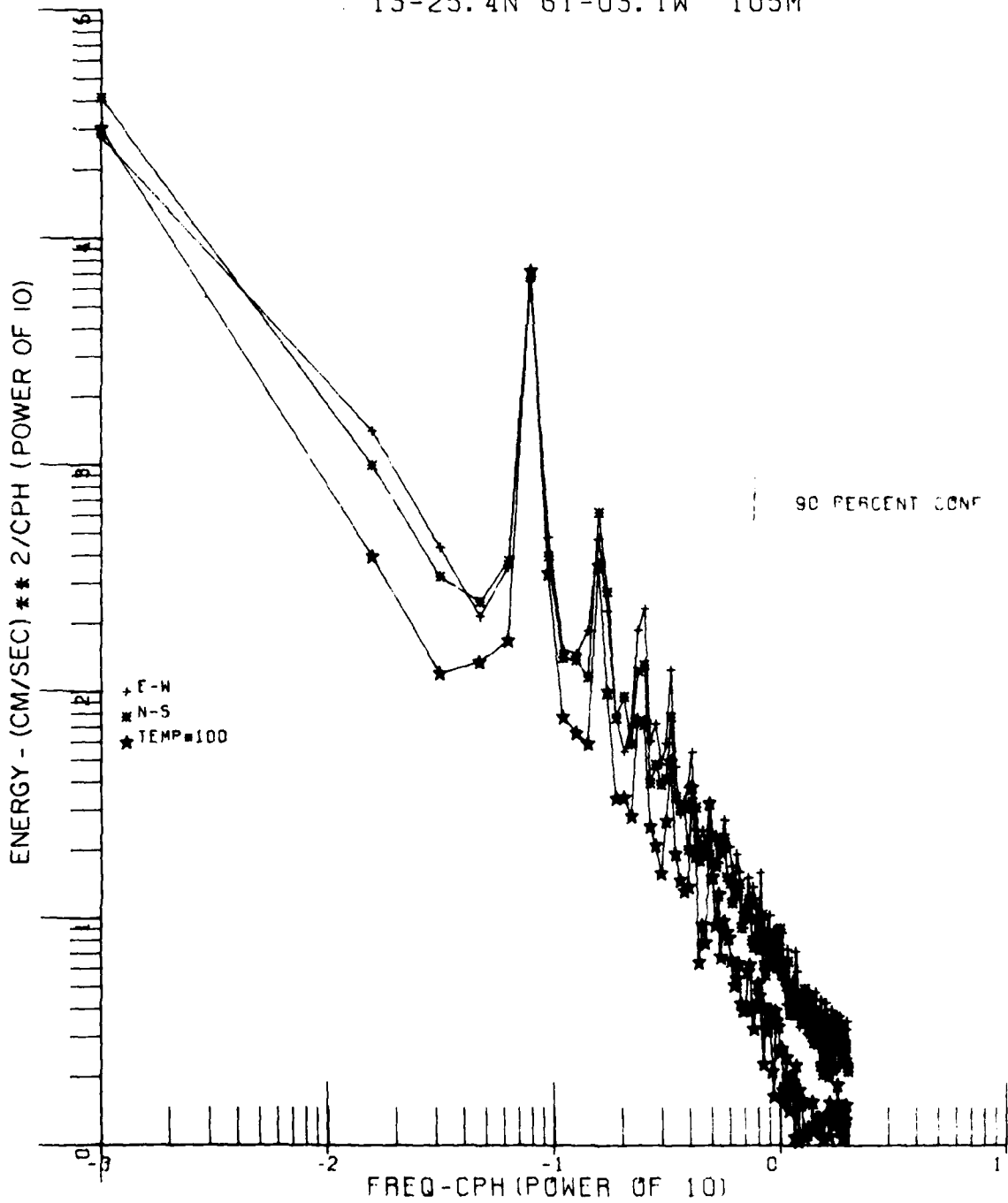
Figure 13. Variance spectra of flow components E (zonal) and N (meridional), and temperature ( T^2/cph ) at 105 m in St. Vincent Passage (array A, see Table 1). Data were not filtered.
