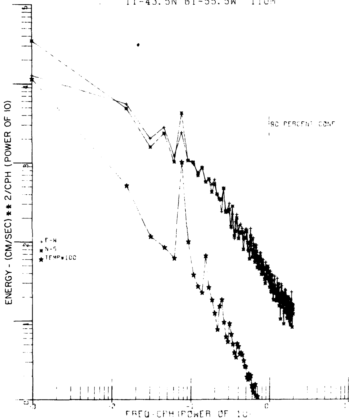
Figure 19. Variance spectra of flow components and temperature ( T^2/cph ) at 110 m in Grenada Passage (see Table 1). Data were not filtered.
