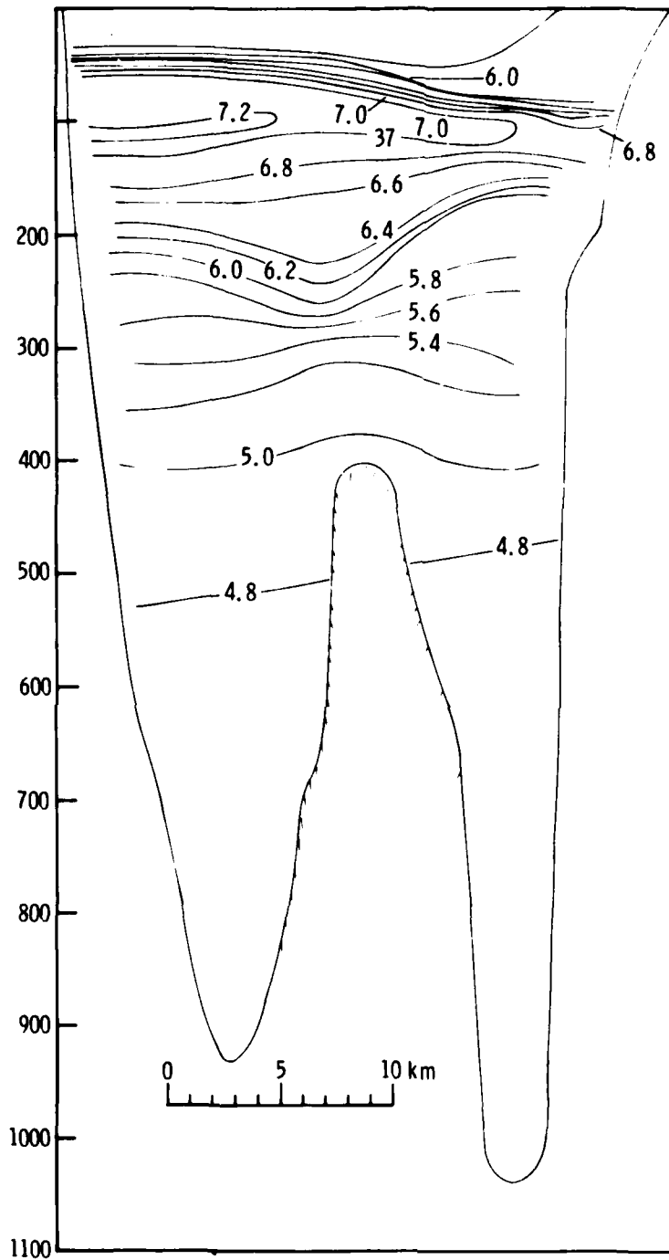
Figure 2b. Vertical salinity (‰) distribution (less 30 ‰) in St. Vincent passage, 3 February 1977.
