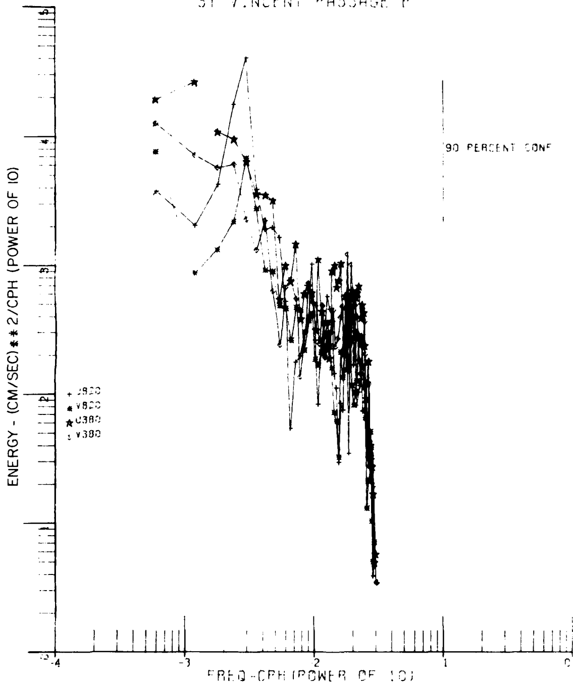
Figure 23. Low frequency variance spectra of E and N components at 380 m and 810 m in St. Vincent Passage (array B, see Table 1).
