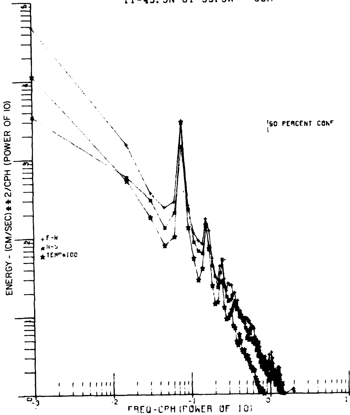
Figure 18. Variance spectra of flow components and temperature ( T^2/cph ) at 60 m in Grenada Passage (see Table 1). Data were not filtered.
