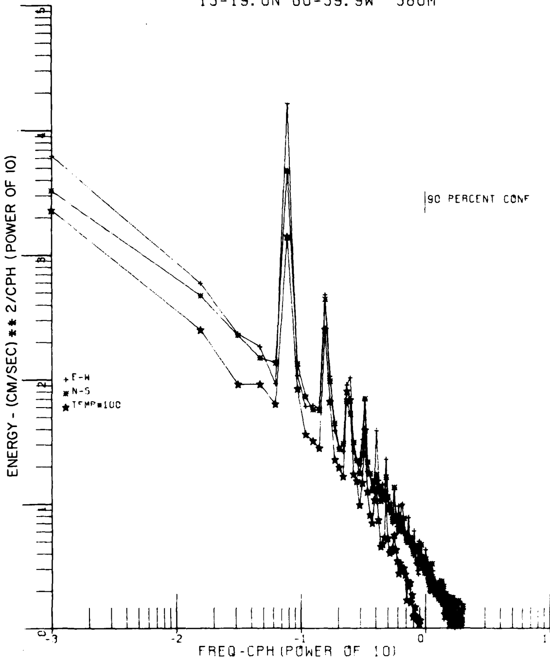
Figure 16. Variance spectra of flow components and temperature (T 2 /cph) at 380 m in St. Vincent Passage (array B, see Table 1). Data were not filtered.
