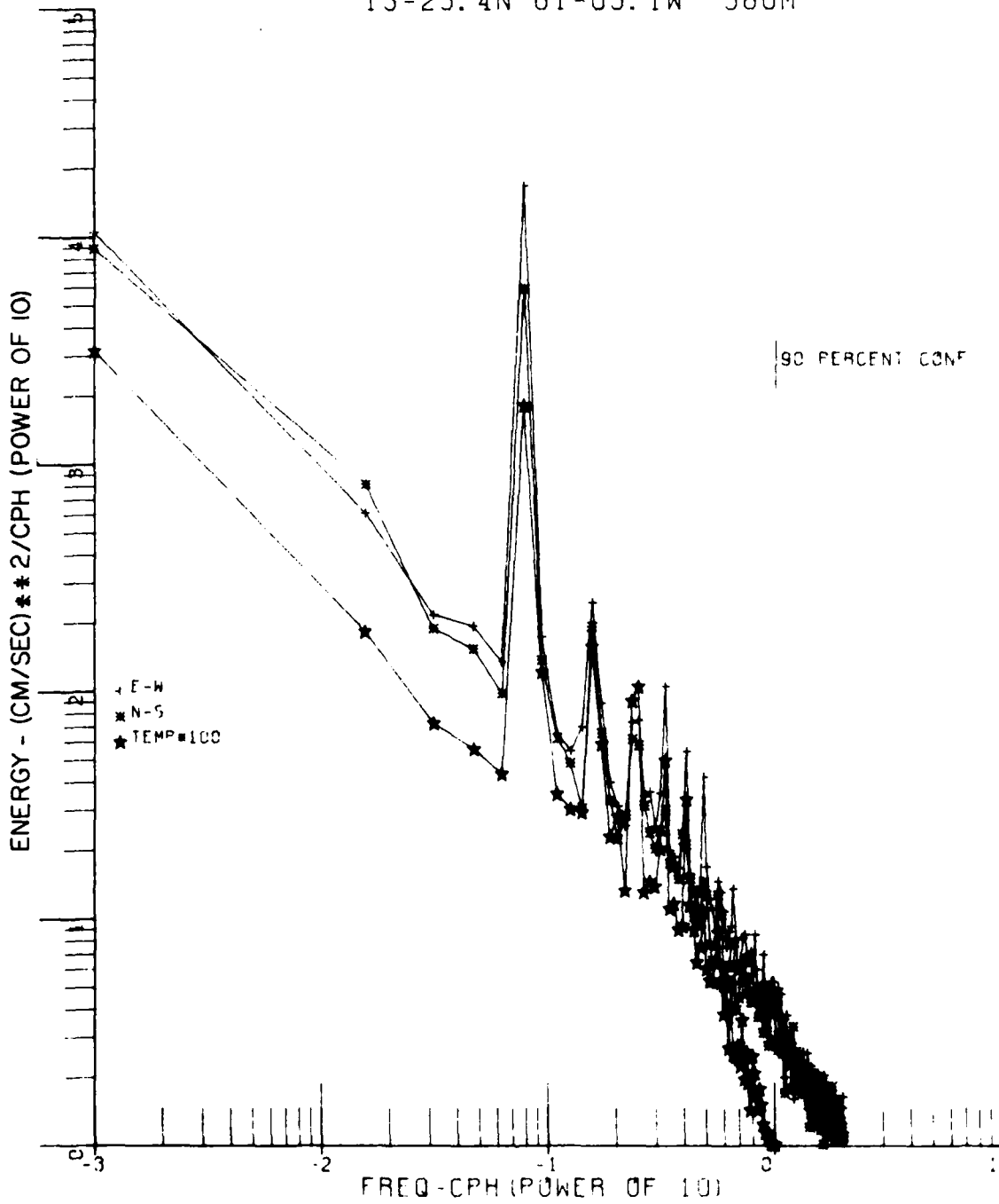
Figure 14. Variance spectra of flow components and temperature ( T^2/cph ), at 380 m in St. Vincent Passage (array A, see Table 1). Data were not filtered.
