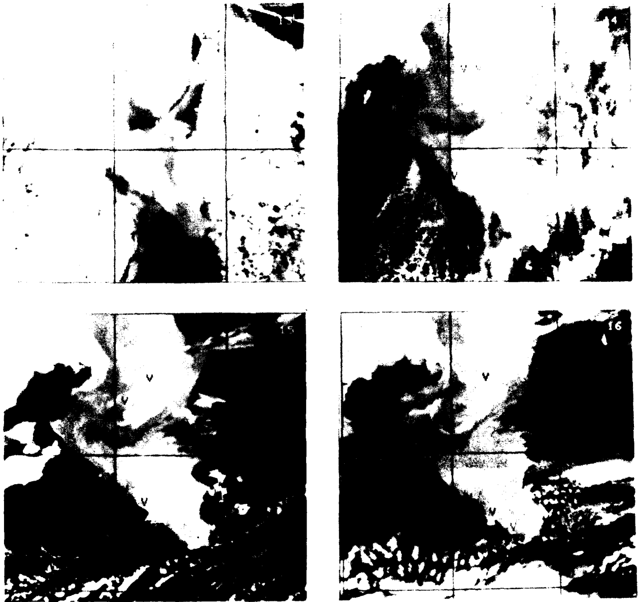
Figure 20. TIROS-N satellite imagery for 13, 14, 15 and 16 May 1979 showing the day-to-day movement of the Southeast Newfoundland Ridge frontal feature. The latitudinal and longitudinal lines form 2^{\circ} squares. Their values may be derived from the 15 May TIROS-N image in Figure 19. The arrows point to identifiable portions of the feature that moved during the four-day period.
