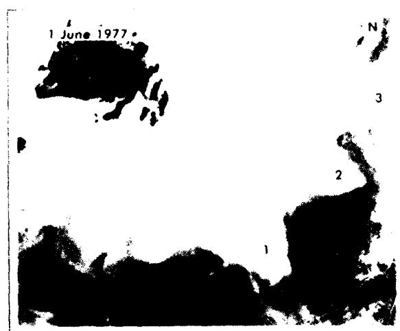
Figure 5. Satellite infrared imagery for the period January 1975 through October 1979 show that three frontal extrusions were always present in the cloud-free data. However, imagery showing all three structures at one time are rare. The ones presented here are meant only as examples of these features. The dark portions of the picture represent warm temperatures, while the light portions represent cold temperatures. The extremely light portions are the cold tops of clouds. Newfoundland is the dark land mass in the upper left corner of each image. The line drawing on the bathymetry chart is a composite of all of the imagery for 1978 drawn by hand on a common grid. The solid line represents the edge of the cold water of the Labrador Front. The dashed line represents the direction and type of extrusion away from the front. The shaded area northwest of the front represents the dominant position of the Labrador Current as seen in the imagery. The smaller shaded areas in the west are smaller slope water current features that also appeared in the 1978 imagery. Composites drawn for other years' imagery show similar results.
