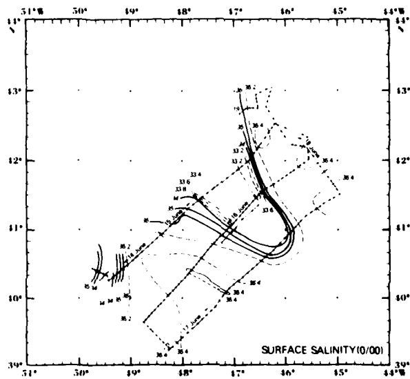
Figure 16. Analysis of surface salinity data collected by the USNS LYNCH from 14 through 18 June 1978.
