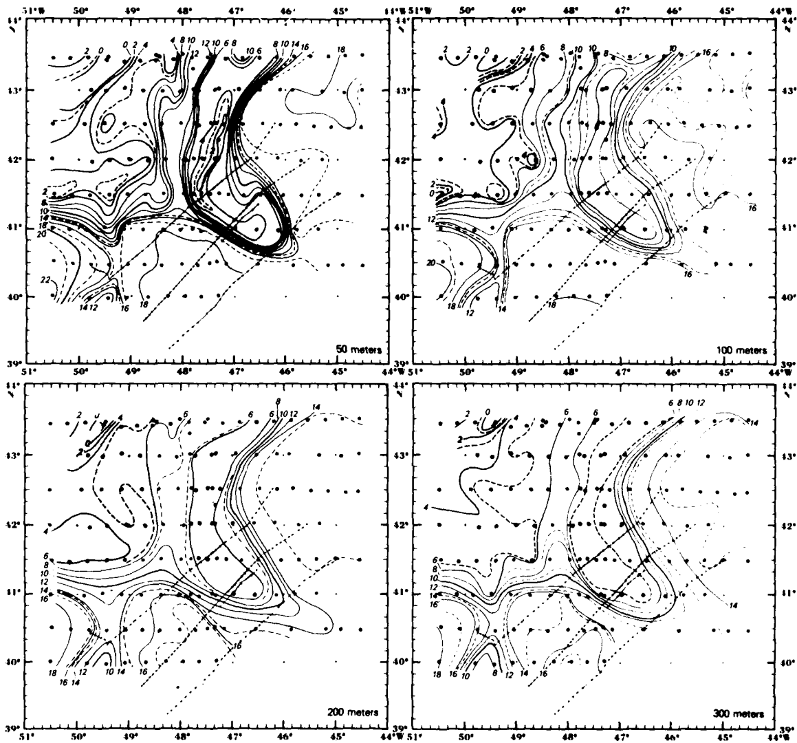
Figure 9. Horizontal analyses in ^{\circ}\text{C} of aircraft 350 m XBT data obtained on 17/18 June. The solid dots refer to the drop locations of the XBTs. The four diagonal lines refer to the drop location of ship and aircraft XBTs whose data are analyzed in the cross-sections in Figures 11 and 14.
