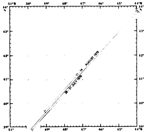
Figure 26. TIROS-N image for 28 July 1979 showing the track of USNS LYNCH for the period 28 through 31 July. The adjacent chart shows the double tracks of the ship in July and August.
