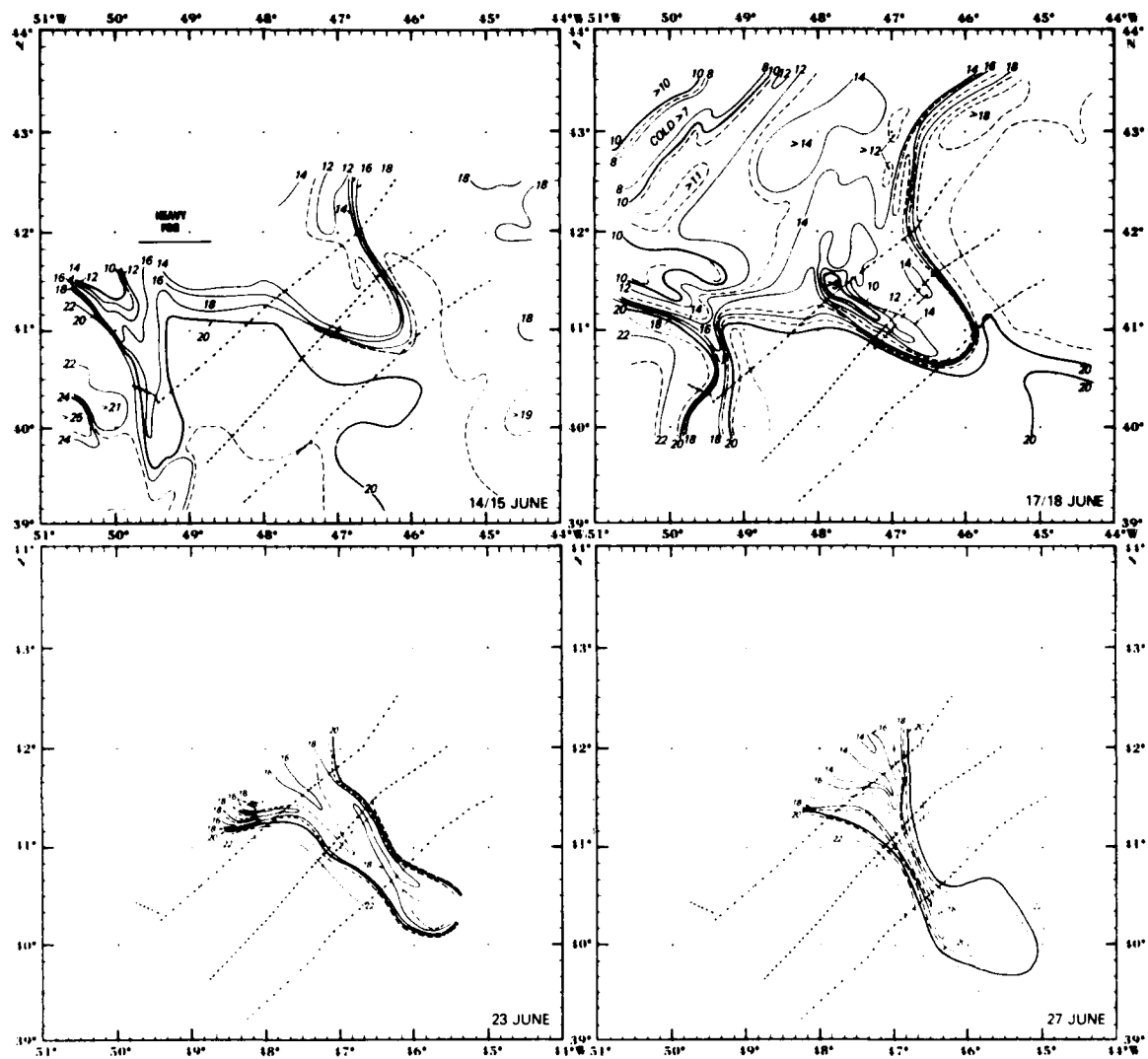
Figure 7. Analyses of aircraft Precision Radiation Temperature (PRT) data in ^{\circ}\text{C} for the ocean surface temperatures during Baseline. The four diagonal lines refer to drop location of ship and aircraft XBTs whose data are analyzed in Figures 11 and 14. In the 14/15 June analysis, the aircraft flew on the western side on 14 June and the eastern side on 15 June. In the 17/18 June analysis the aircraft flew the western side of the Figure on 18 June and the eastern side on 17 June. In flying the western and eastern flight tracks, a 50 km overlap was maintained.
