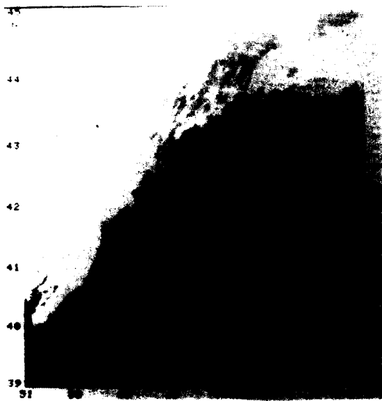
Figure 26. TIROS-N image for 28 July 1979 showing the track of USNS LYNCH for the period 28 through 31 July. The adjacent chart shows the double tracks of the ship in July and August.
