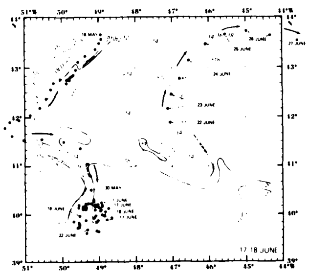
Figure 17. Movement of satellite drifter buoys within the Grand Banks Experiment area during Baseline (Richardson, 1980). The drifter buoy in (a) was released by the USCGC EVERGREEN on 13 April; the buoy in (b) was released by the USNS LYNCH on 22 June. The dots represent positions at time intervals of approximately twice a day (1200 and 2400 GMT). The 17/18 June PRT analysis is presented to give perspective to the position of the thermal gradients during a portion of the buoy's movement. The entire track of the western buoy in (a) may be further compared to the position of the Labrador Current shown as the cold north-south sinuous feature in the lower section of the 12 June satellite image in Figure 6. The entire track of the eastern buoy may be compared to the position of the northern of the two extrusions in the 25 June image of Figure 6.
