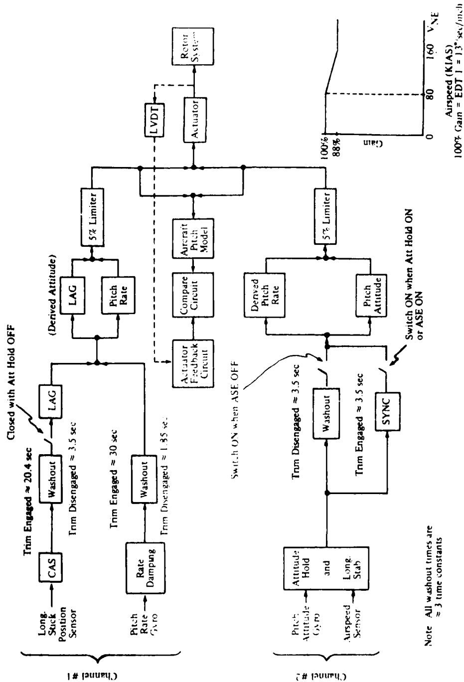
Figure 8. Pitch SAS
