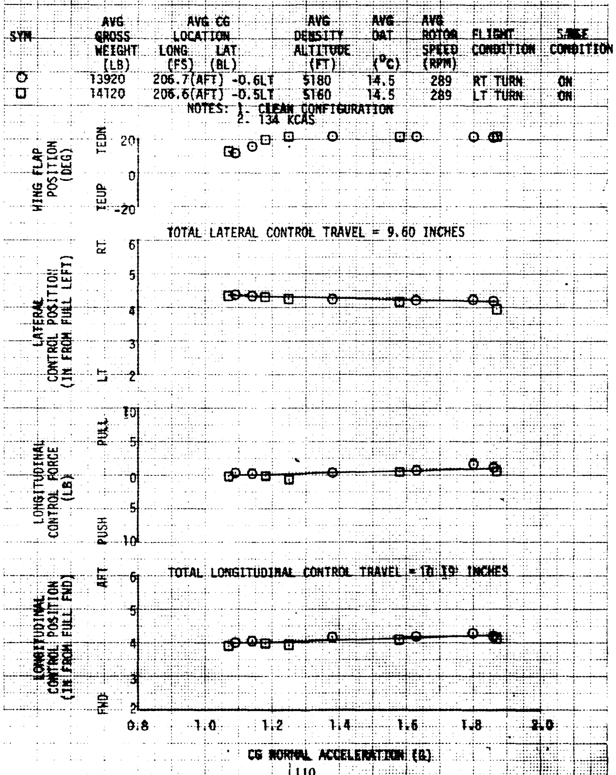
FIGURE 27 MANEUVERING STABILITY YAH-64 USA S/N 74-22248
