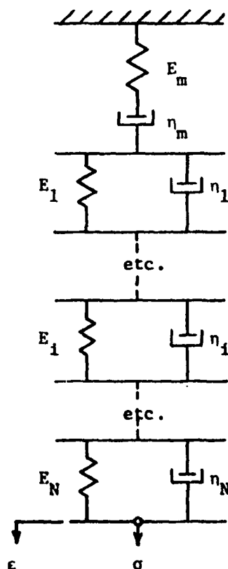
Figure 8. Kelvin Model
