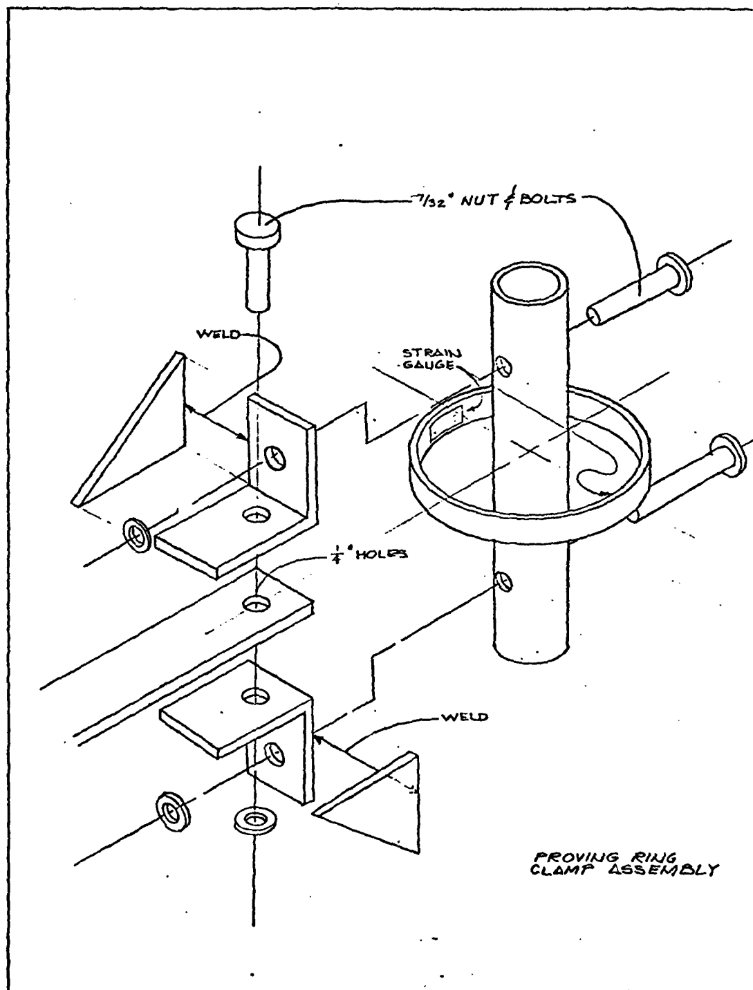
Figure 53. Diagram of a Proving Ring Load Cell From the Biaxial Strain Tester.
