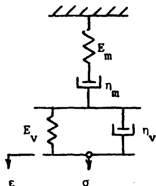
Figure 6. Series Arrangement of Maxwell and Voigt Models
