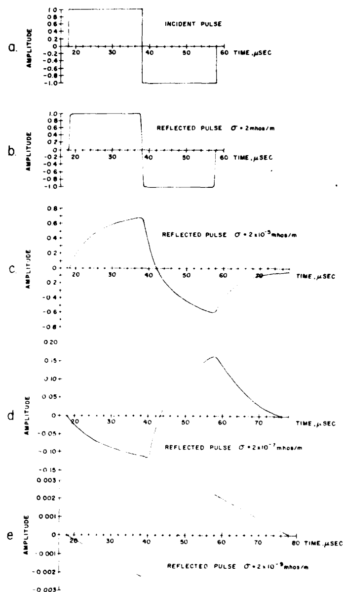
Figure 14. Slab TM Reflections of Single-Cycle Square-Wave Pulses. (a) Incident pulses, (b) reflected pulses, \sigma = 2 \text{ mho/m} , (c) reflected pulse, \sigma = 2 \times 10^{-5} \text{ mho/m} , (d) reflected pulse, \sigma = 2 \times 10^{-7} \text{ mho/m} , (e) reflected pulse, \sigma = 2 \times 10^{-9} \text{ mho/m} . In all cases the incidence angle is 60^\circ and the slab thickness is 6 \text{ km}
