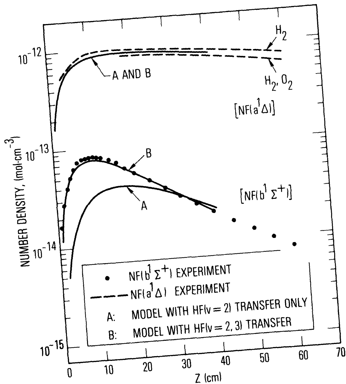
Fig. 4. Model Fit of \text{NF}(b^1\Sigma^+) Density vs. Axial Position Z
