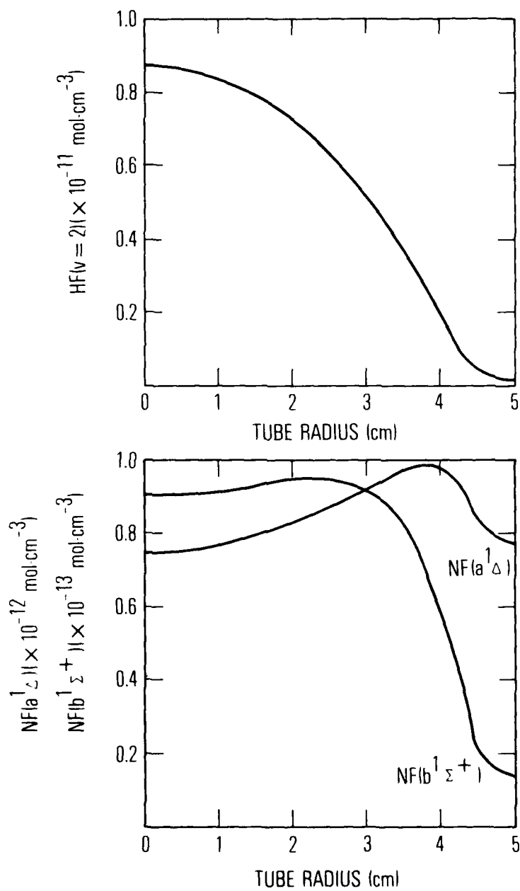
Fig. 2. Radial Variations of Selected Species at Z = 10 \text{ cm}
