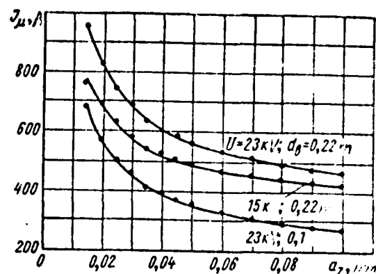
Fig. 3. Value of magnetizing current as a function of the axial dimension of the inductor's core at various values of pulsed voltage and internal diameter of the core.
