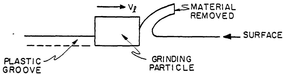
(b) PLASTIC GROOVING MECHANISM
