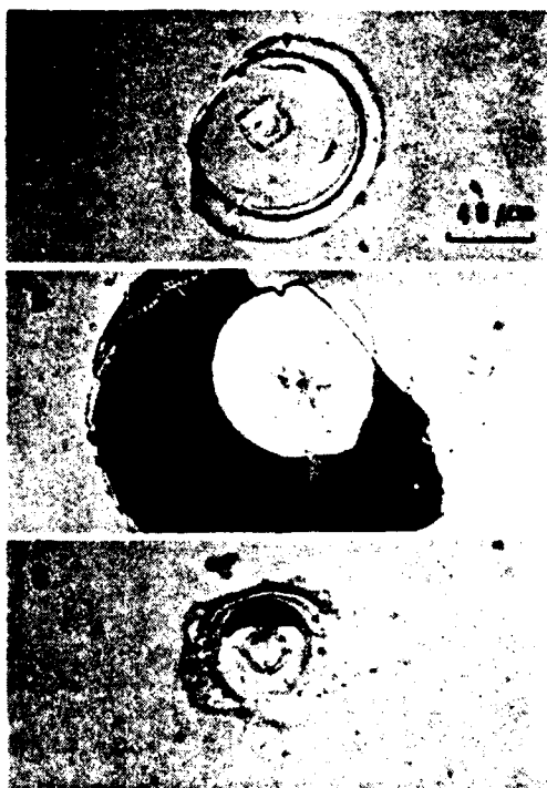
Fig. 8. Optical micrographs indicating variations in the lateral crack size for a sample indented at different locations. This film exhibits poor and variable adhesion.
