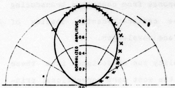
Fig. 1-8. Measured directivity pattern for 0.42cm diameter (equivalent to half wavelength at 167 kHz in water) circular zinc oxide transducing 10 micron-thick film on 0.002 inch thick stainless steel, measured in water bath with 167 kHz signals. Solid curve is plot of equation \cos\theta \cos \frac{2\theta}{2} \left| \frac{J_1(Ka \sin\theta)}{Ka \sin\theta} \right| where a =radius of the circular aperture; K =wave number in water. Data points indicated by points with error bar.
