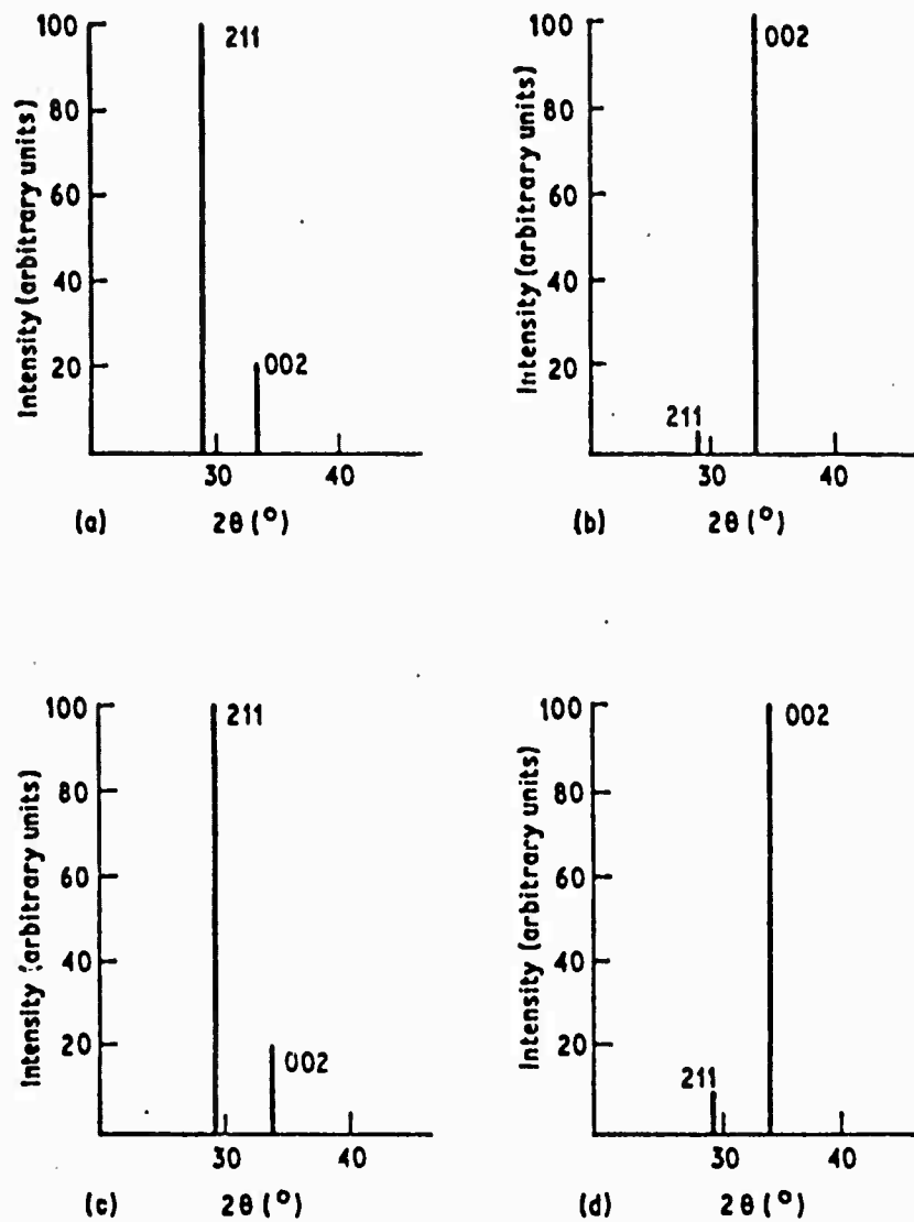
Figure 3 X-ray diffraction patterns of (a) \text{Ba}_2\text{Ge}_2\text{TiO}_6 standard powder diffraction pattern, (b) BTG glass-ceramic, (c) \text{Ba}_2\text{TiSi}_2\text{O}_6 standard powder diffraction pattern, and (d) BTS glass-ceramic.
